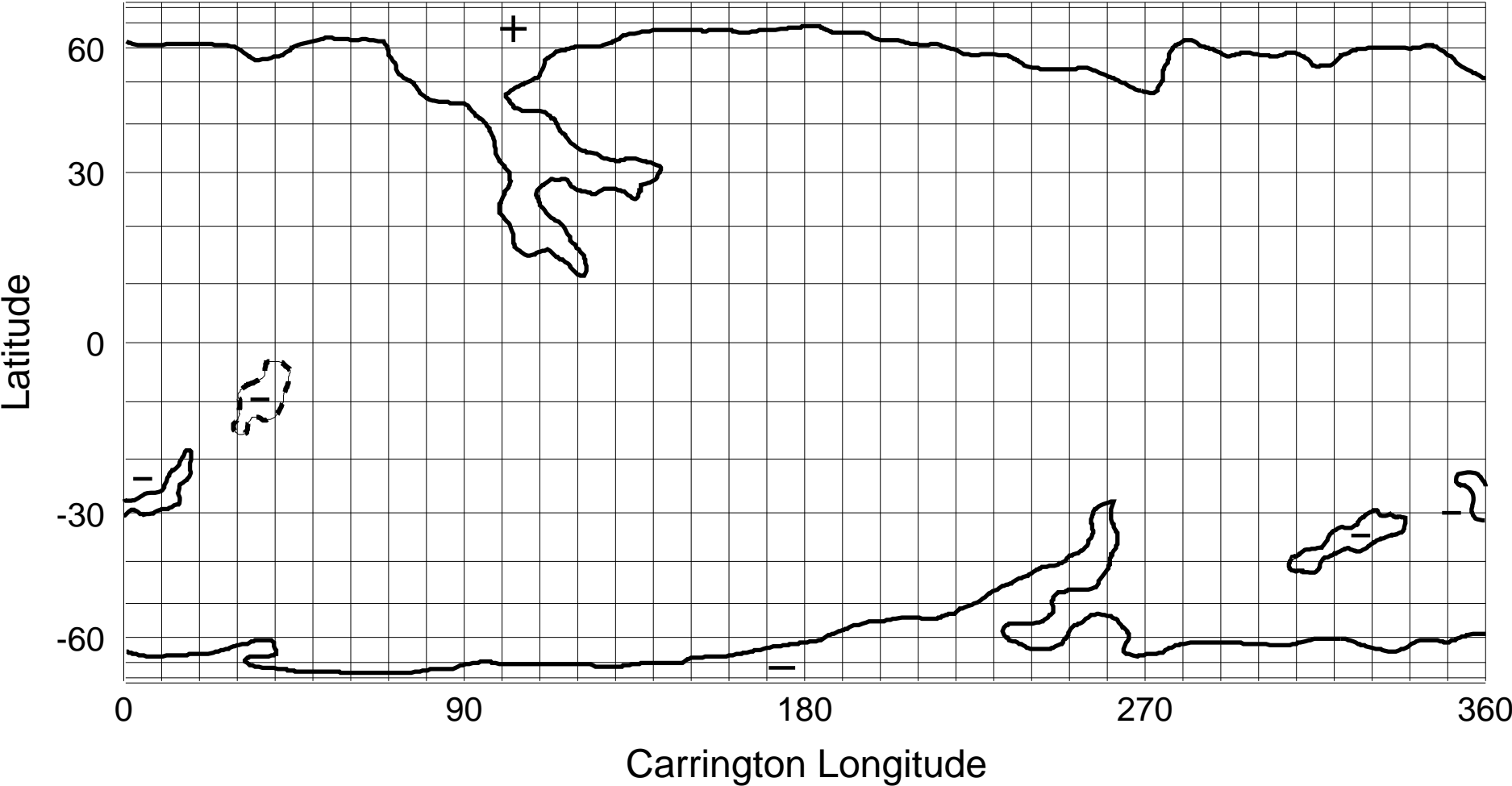
NSO/KP He I 1083 nm Coronal Hole Map: Carrington Rotation 1886
