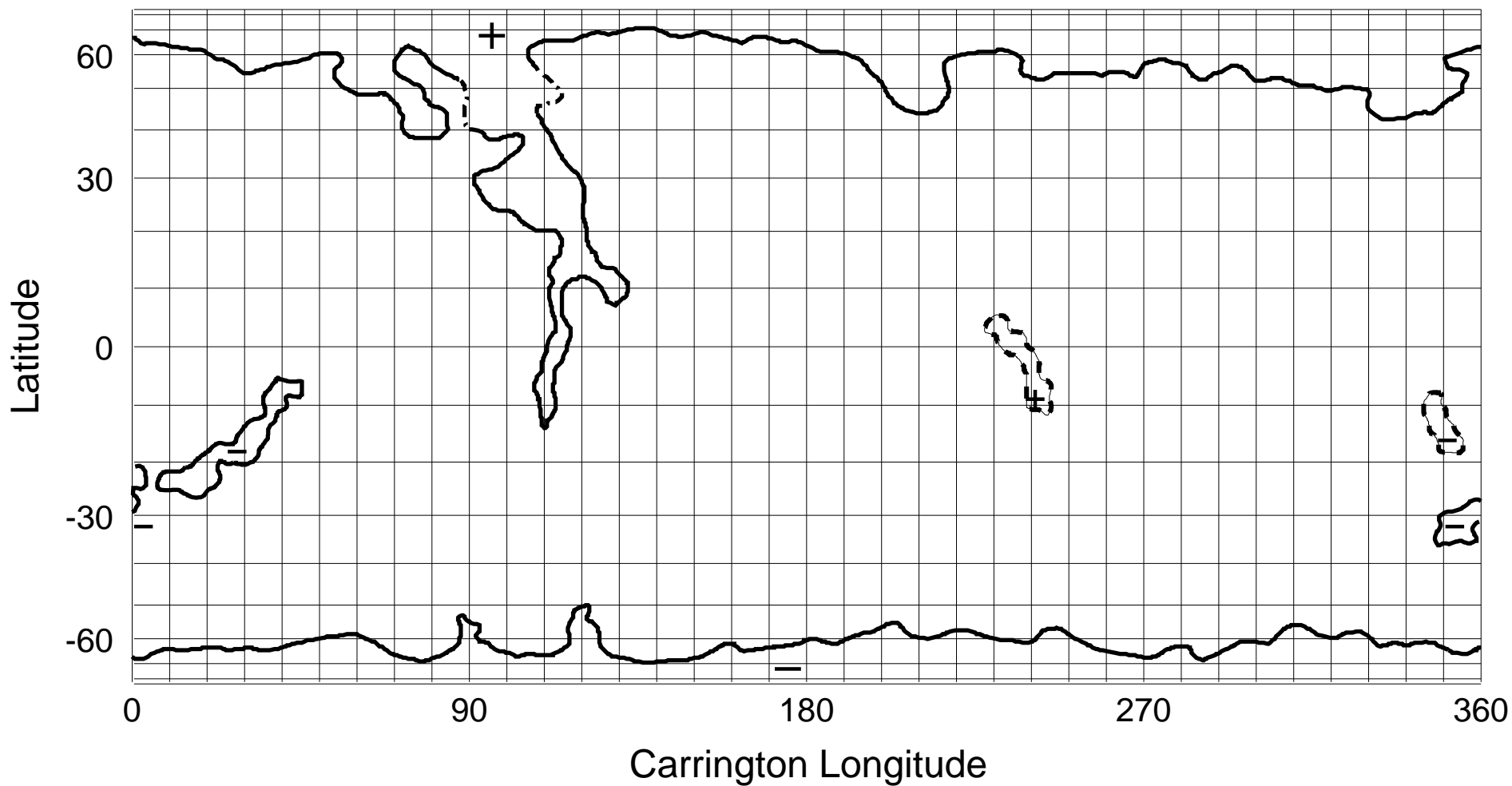
NSO/KP He I 1083 nm Coronal Hole Map: Carrington Rotation 1887
