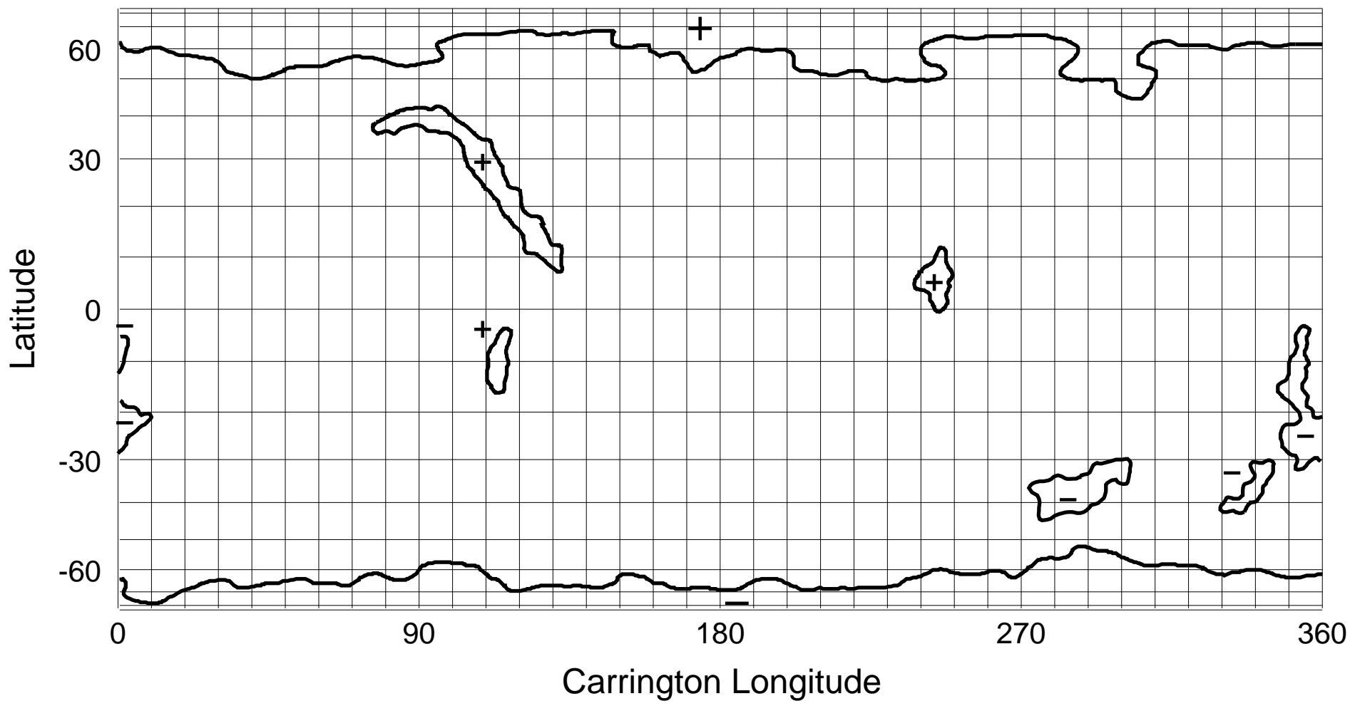
NSO/KP He I 1083 nm Coronal Hole Map: Carrington Rotation 1888
