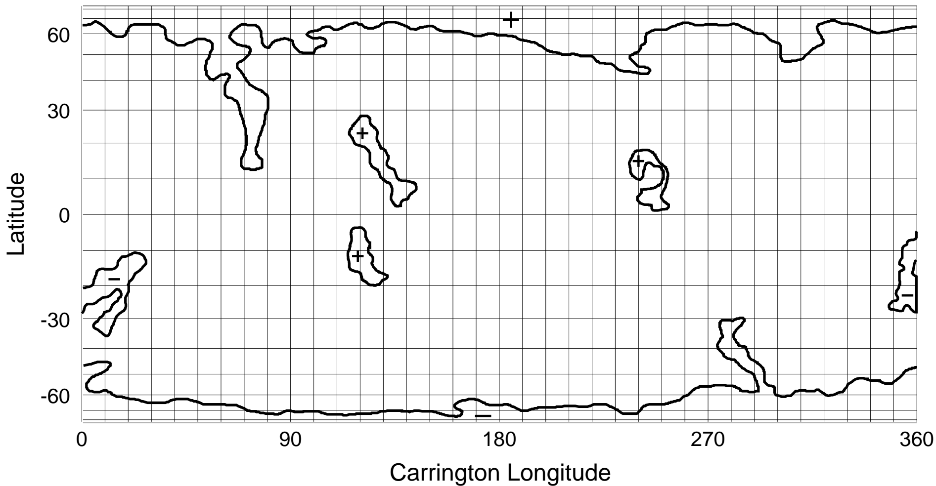
NSO/KP He I 1083 nm Coronal Hole Map: Carrington Rotation 1889
