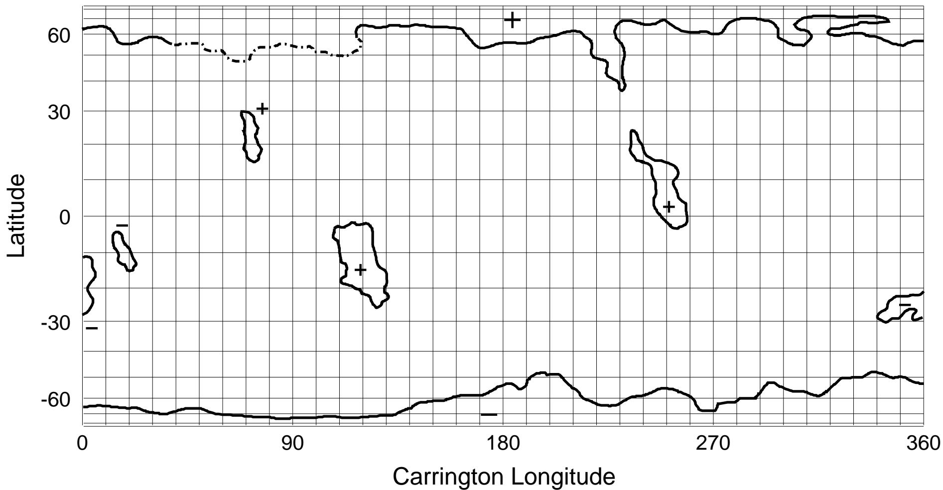
NSO/KP He I 1083 nm Coronal Hole Map: Carrington Rotation 1890
