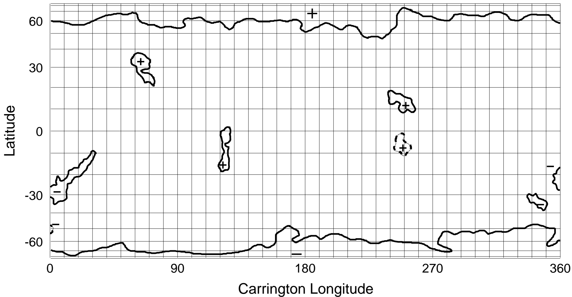
NSO/KP He I 1083 nm Coronal Hole Map: Carrington Rotation 1891
