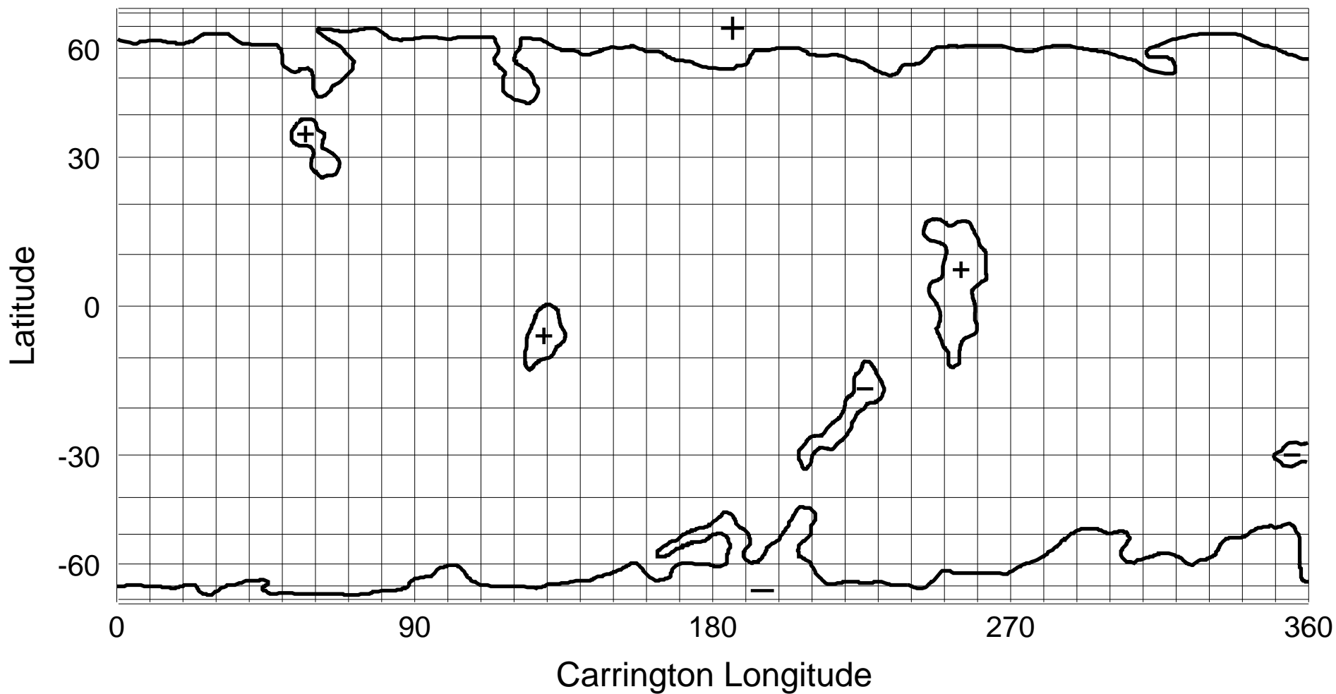
NSO/KP He I 1083 nm Coronal Hole Map: Carrington Rotation 1892
