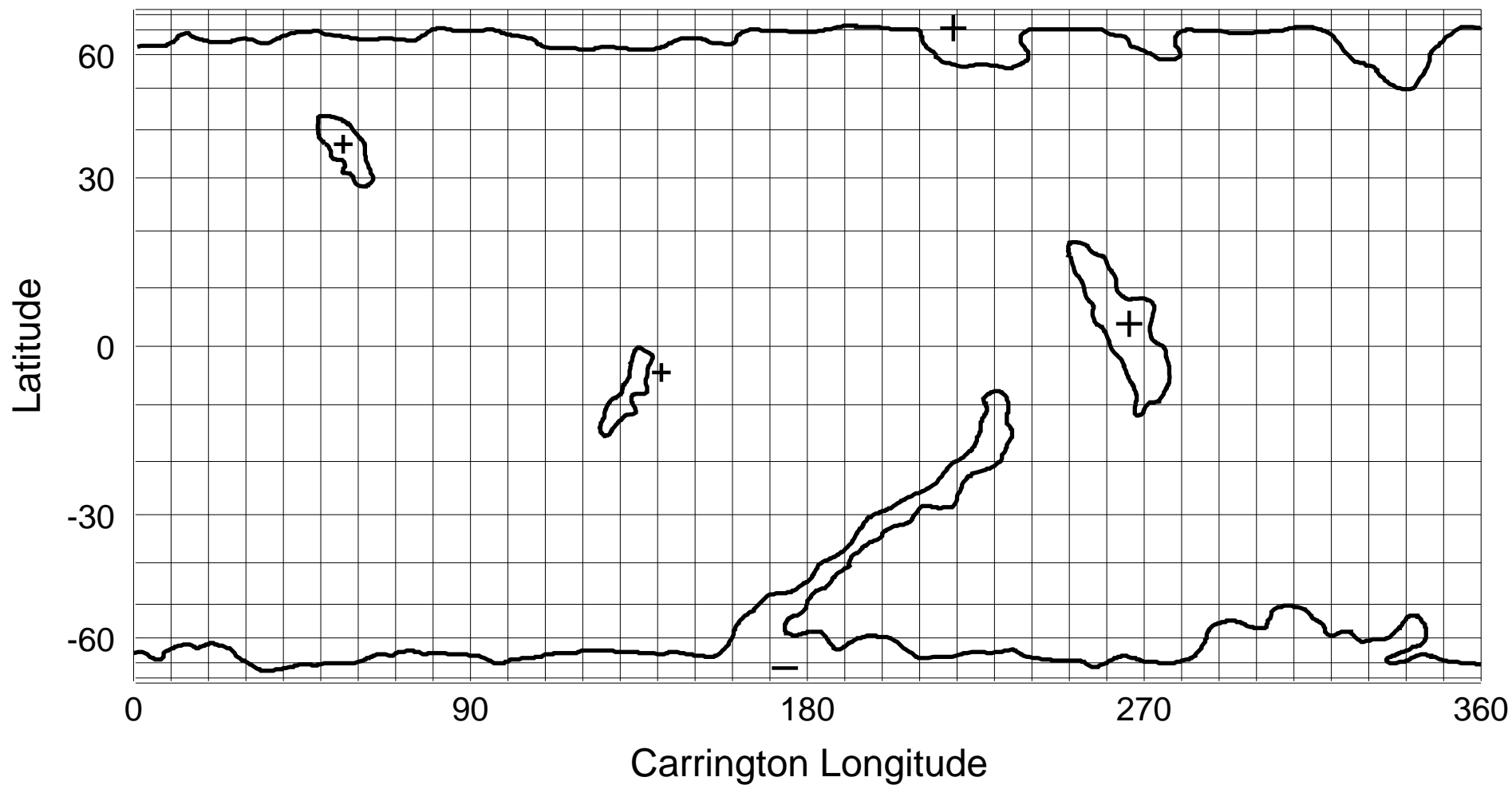
NSO/KP He I 1083 nm Coronal Hole Map: Carrington Rotation 1893
