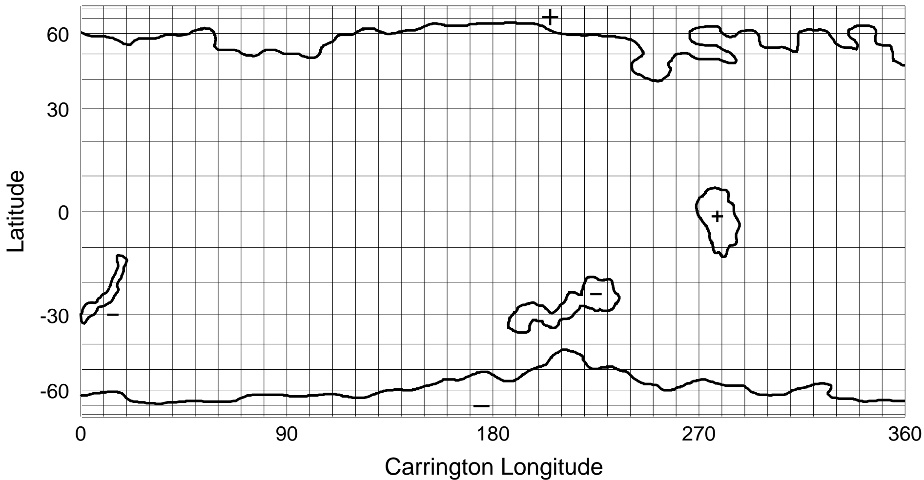
NSO/KP He I 1083 nm Coronal Hole Map: Carrington Rotation 1894
