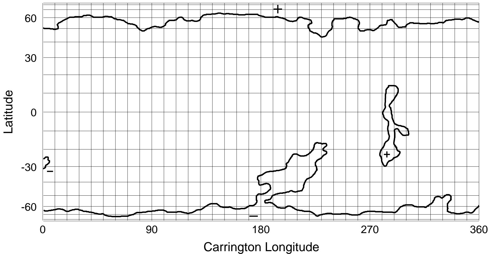
NSO/KP He I 1083 nm Coronal Hole Map: Carrington Rotation 1896
