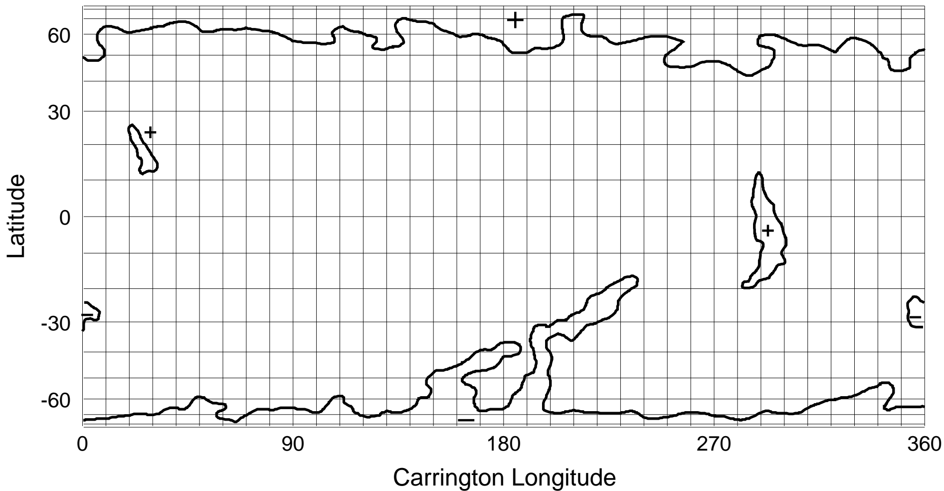
NSO/KP He I 1083 nm Coronal Hole Map: Carrington Rotation 1897
