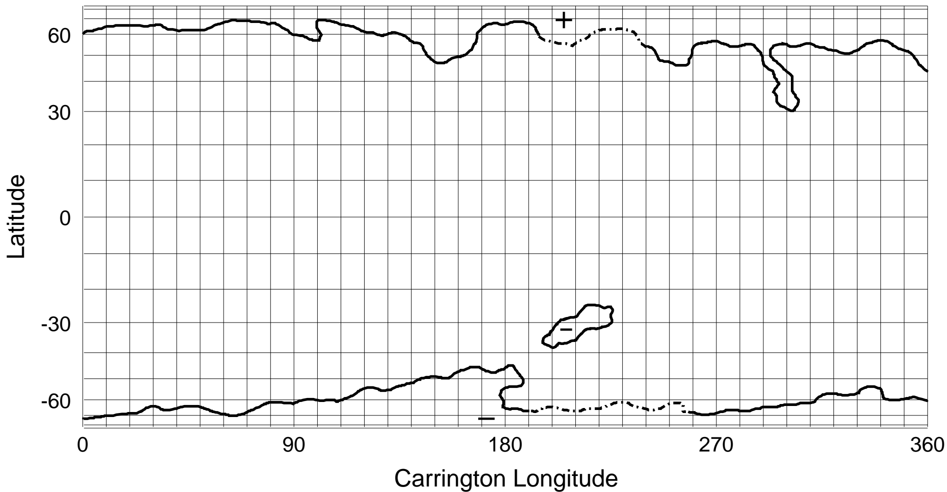
NSO/KP He I 1083 nm Coronal Hole Map: Carrington Rotation 1899
