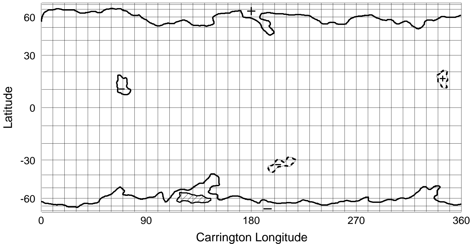
NSO/KP He I 1083 nm Coronal Hole Map: Carrington Rotation 1900
