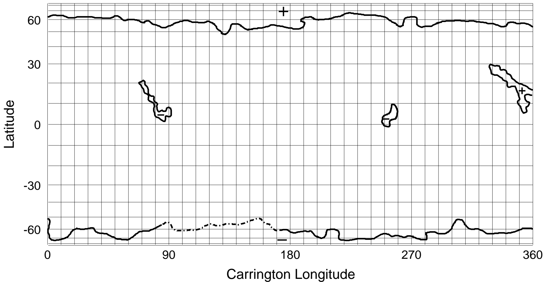
NSO/KP He I 1083 nm Coronal Hole Map: Carrington Rotation 1902
