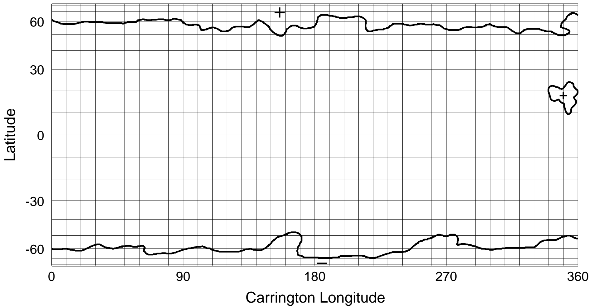
NSO/KP He I 1083 nm Coronal Hole Map: Carrington Rotation 1903
