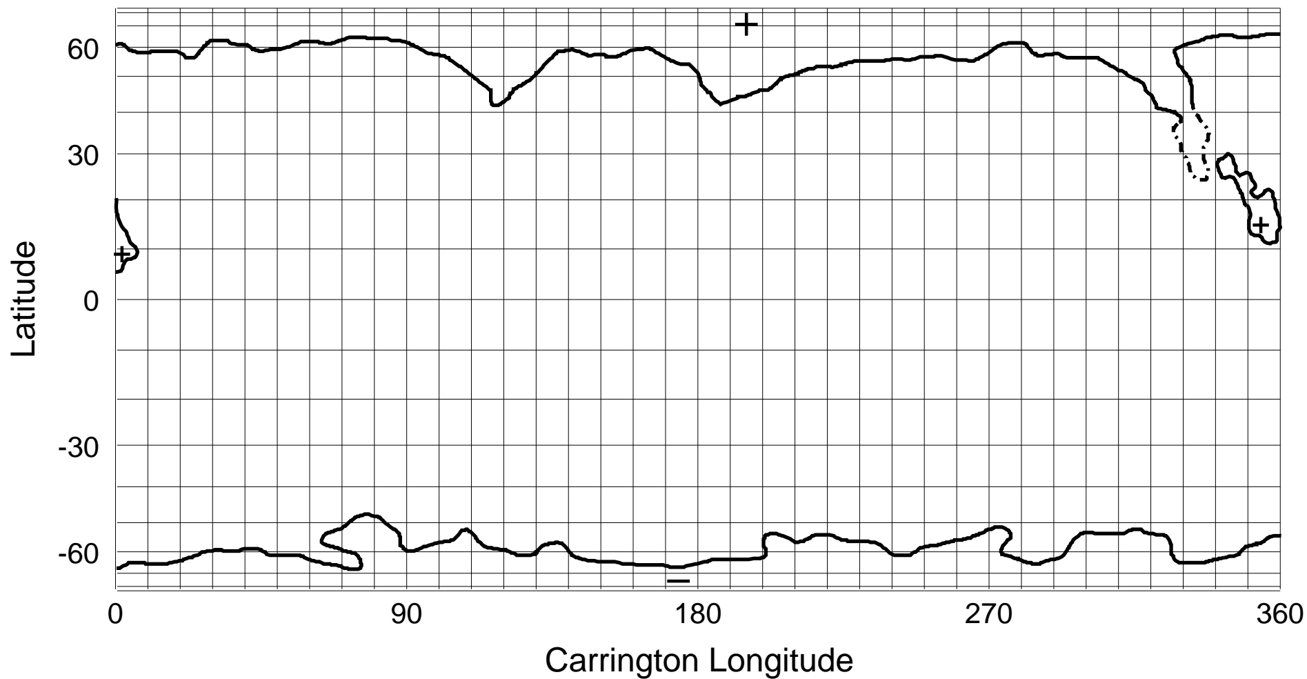
NSO/KP He I 1083 nm Coronal Hole Map: Carrington Rotation 1904
