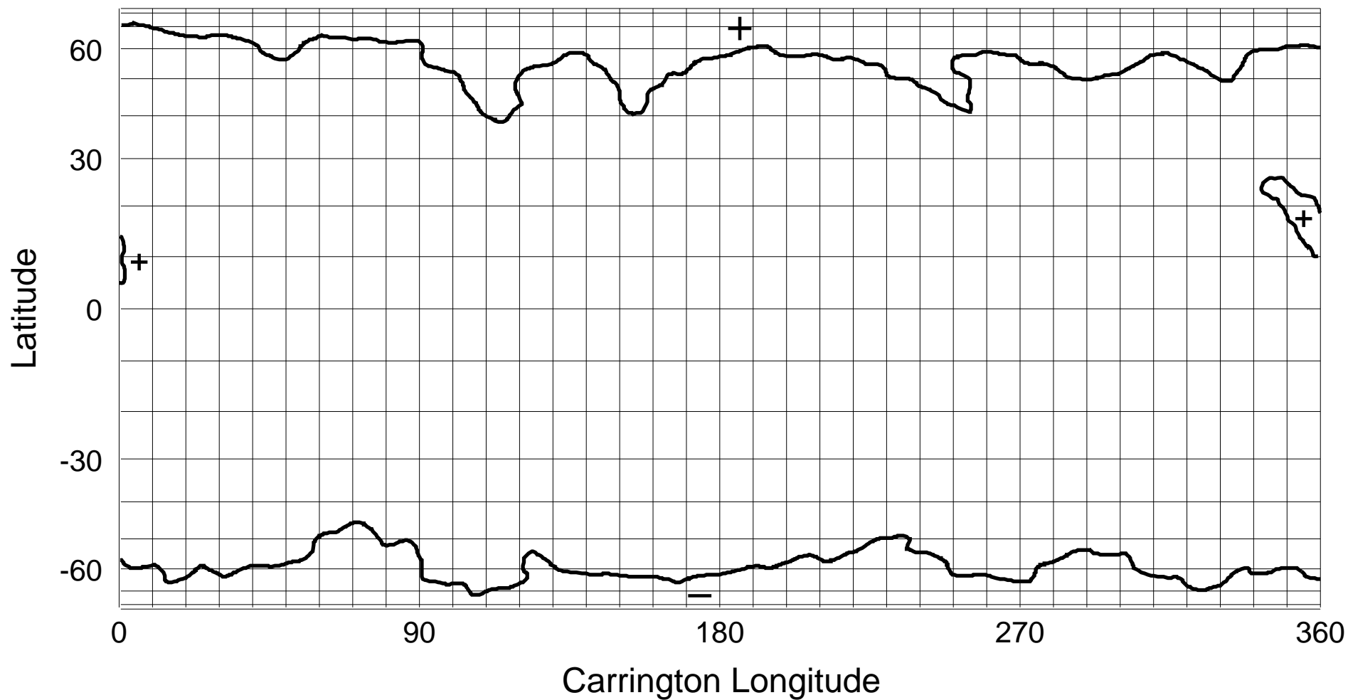
NSO/KP He I 1083 nm Coronal Hole Map: Carrington Rotation 1905
