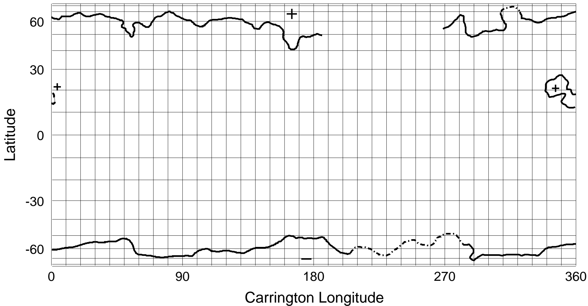
NSO/KP He I 1083 nm Coronal Hole Map: Carrington Rotation 1906
