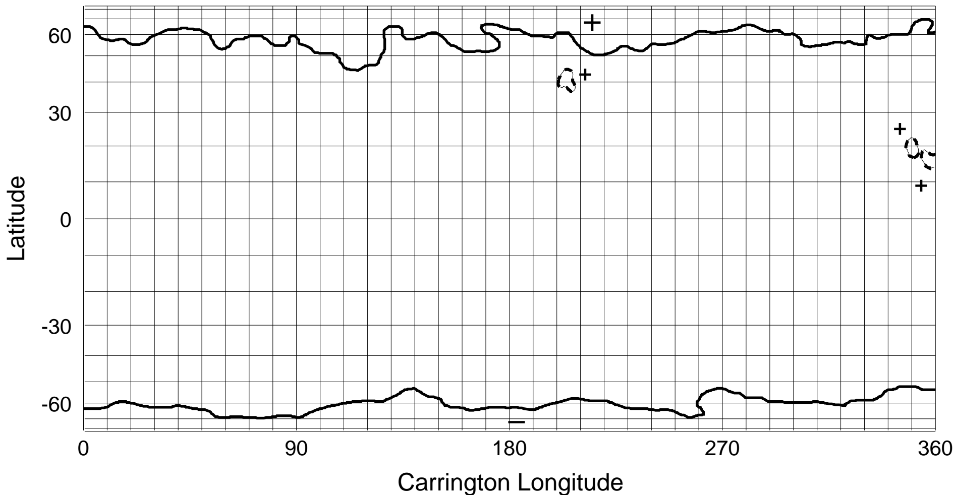
NSO/KP He I 1083 nm Coronal Hole Map: Carrington Rotation 1907
