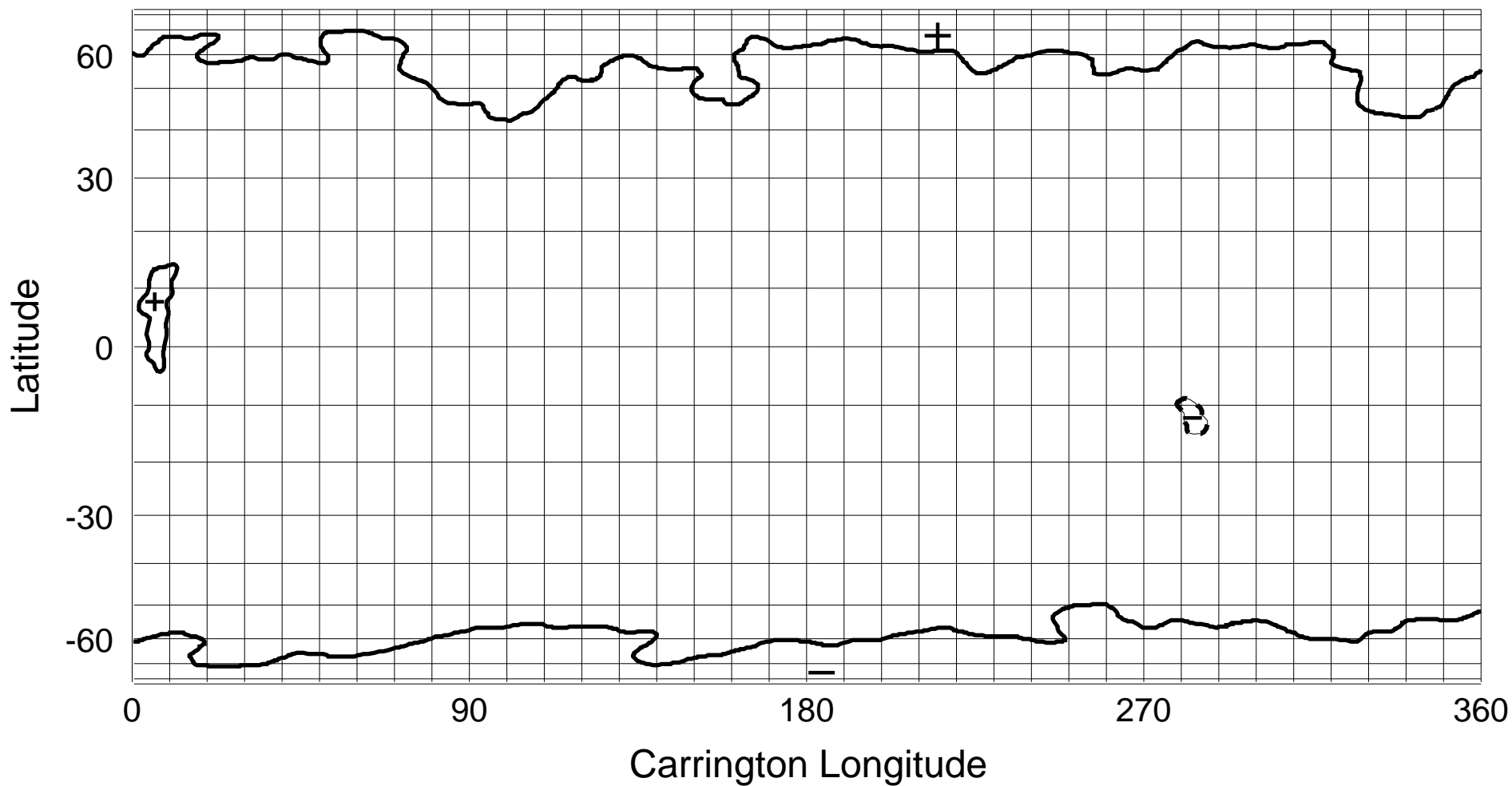
NSO/KP He I 1083 nm Coronal Hole Map: Carrington Rotation 1908
