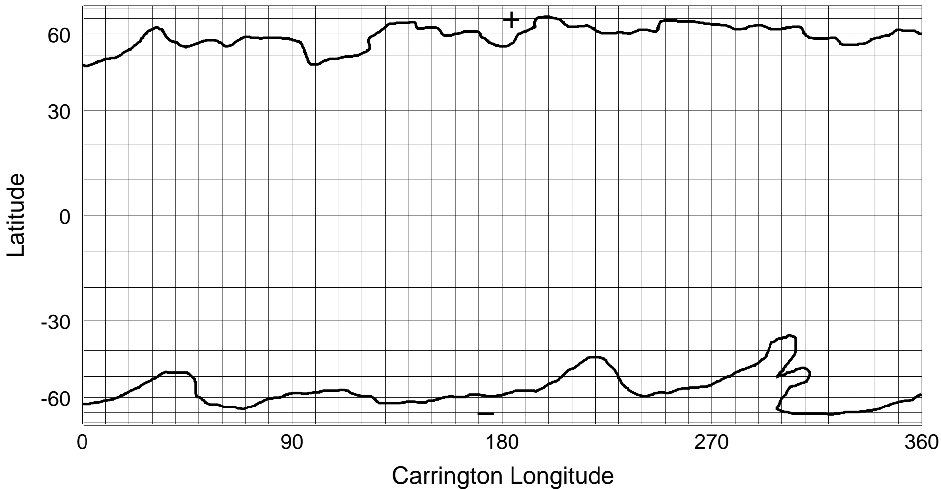
NSO/KP He I 1083 nm Coronal Hole Map: Carrington Rotation 1909
