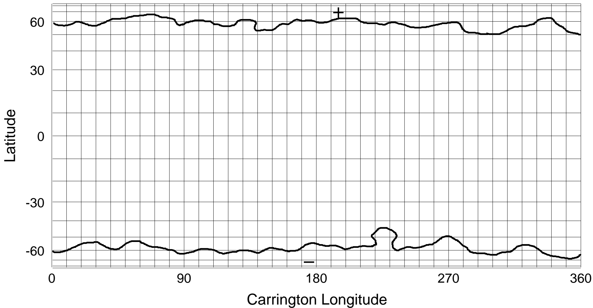
NSO/KP He I 1083 nm Coronal Hole Map: Carrington Rotation 1910
