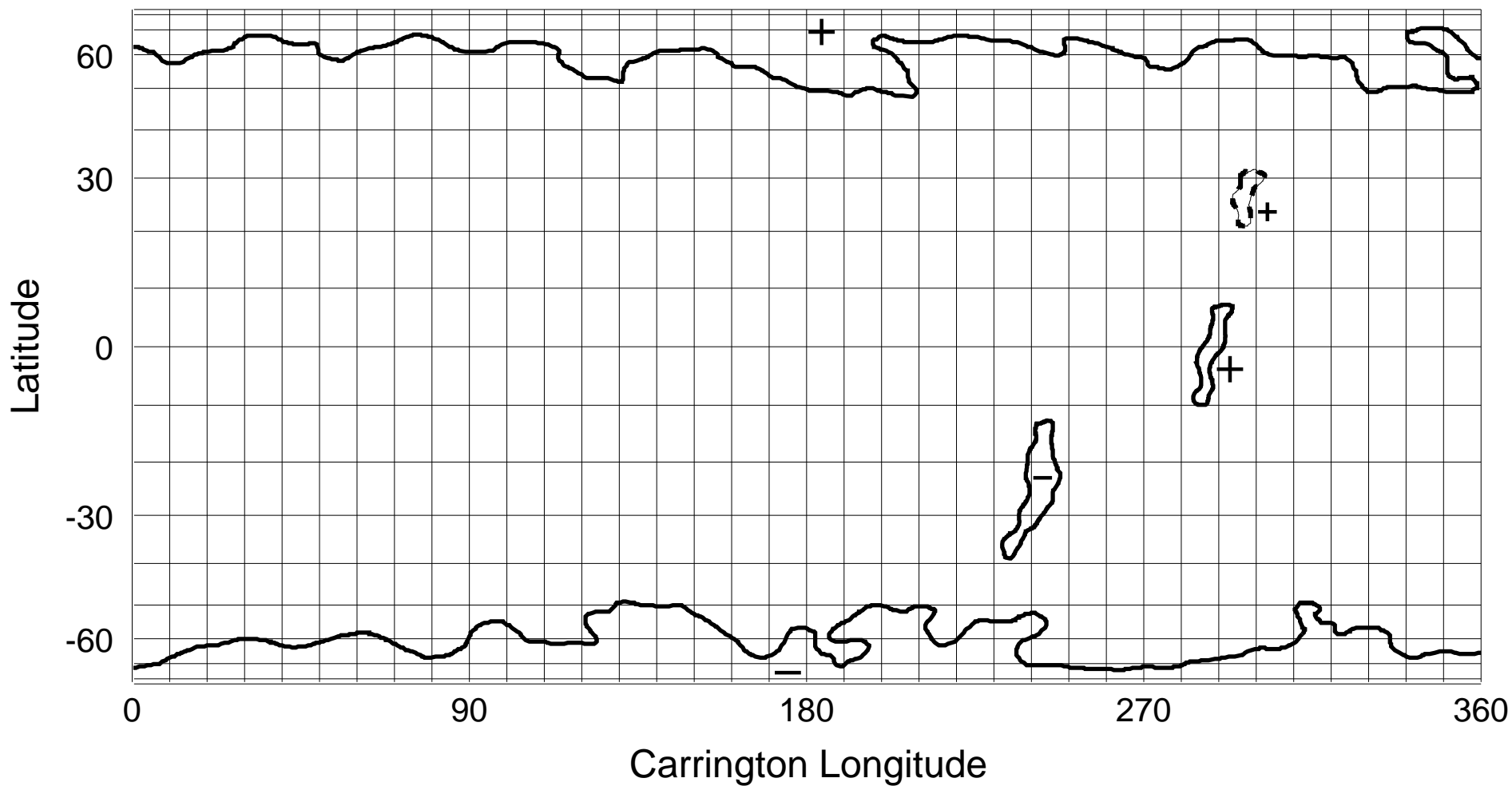
NSO/KP He I 1083 nm Coronal Hole Map: Carrington Rotation 1912
