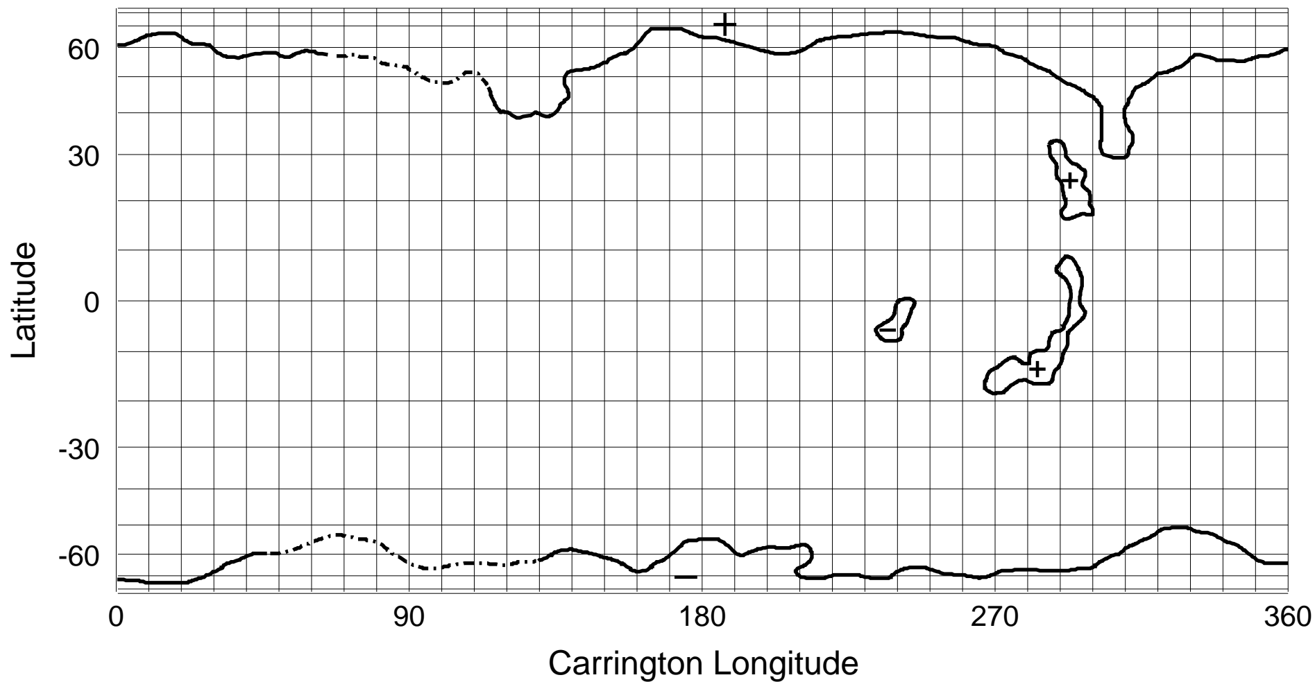
NSO/KP He I 1083 nm Coronal Hole Map: Carrington Rotation 1913
