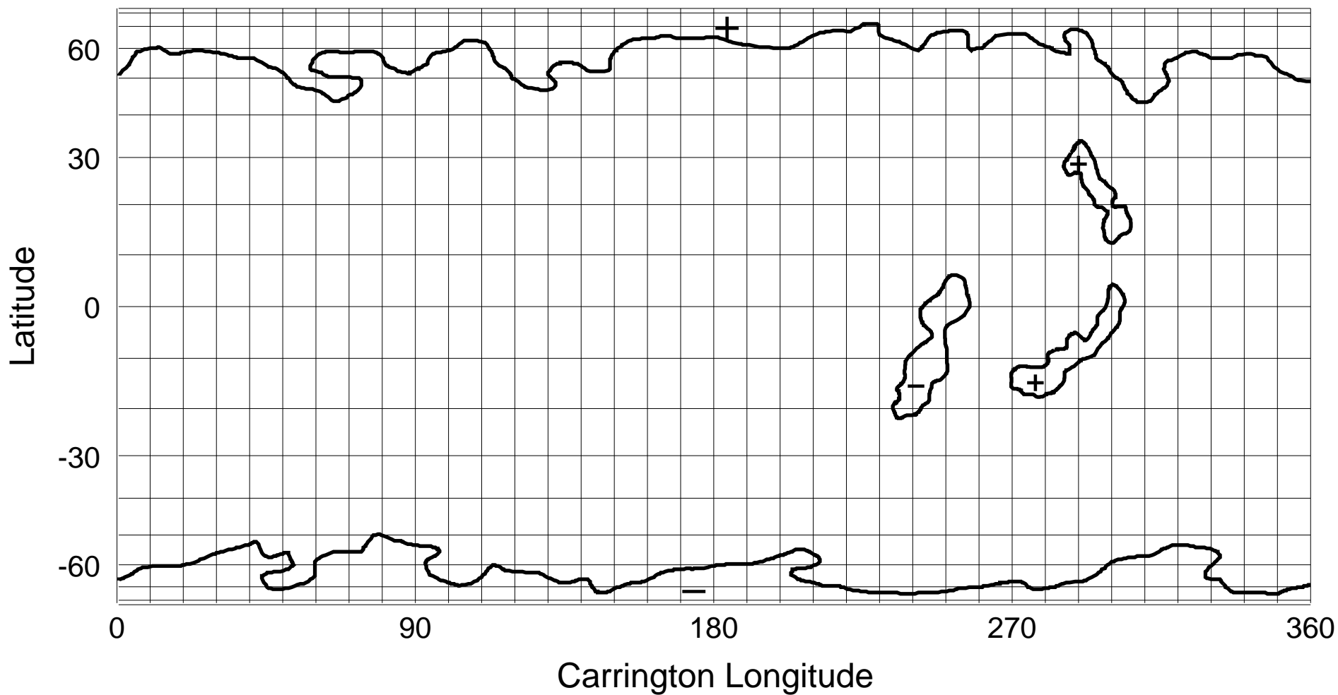
NSO/KP He I 1083 nm Coronal Hole Map: Carrington Rotation 1914
