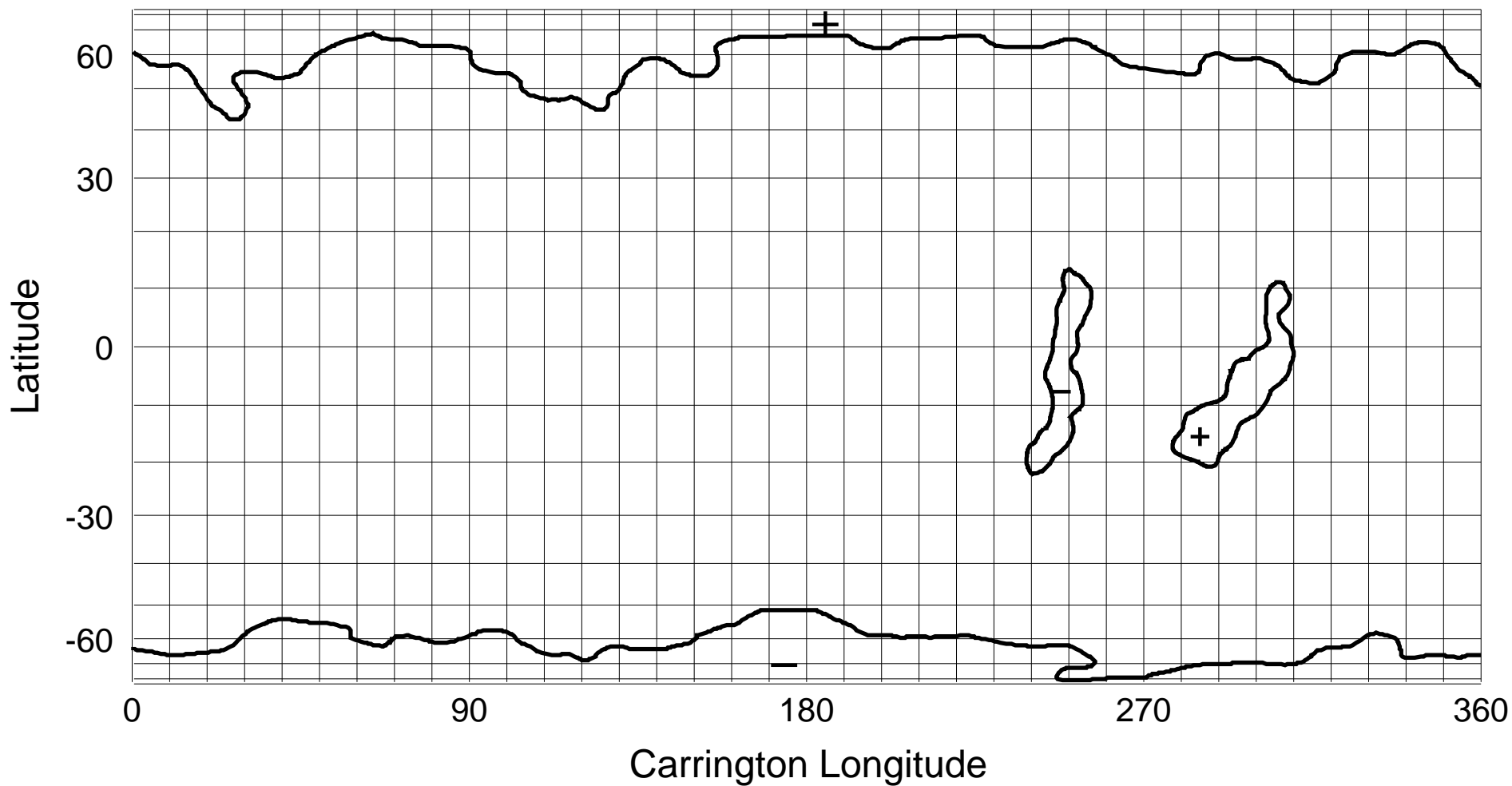
NSO/KP He I 1083 nm Coronal Hole Map: Carrington Rotation 1915
