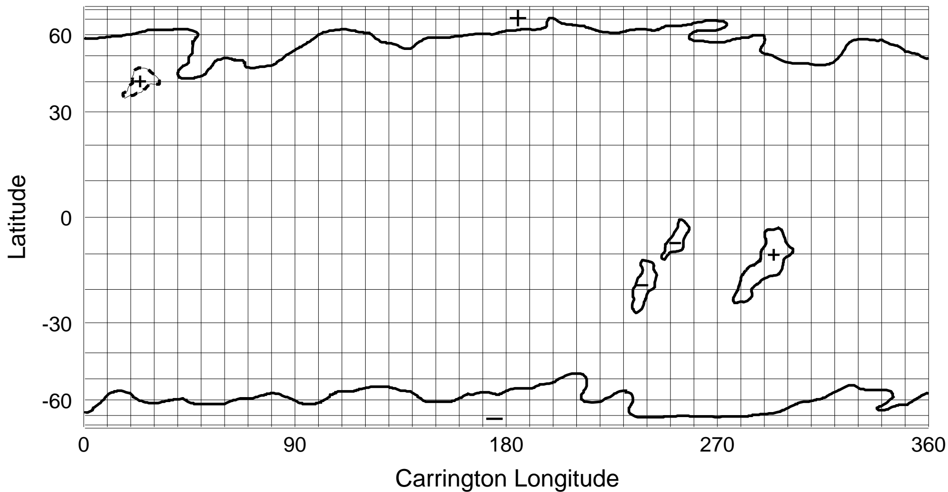
NSO/KP He I 1083 nm Coronal Hole Map: Carrington Rotation 1916
