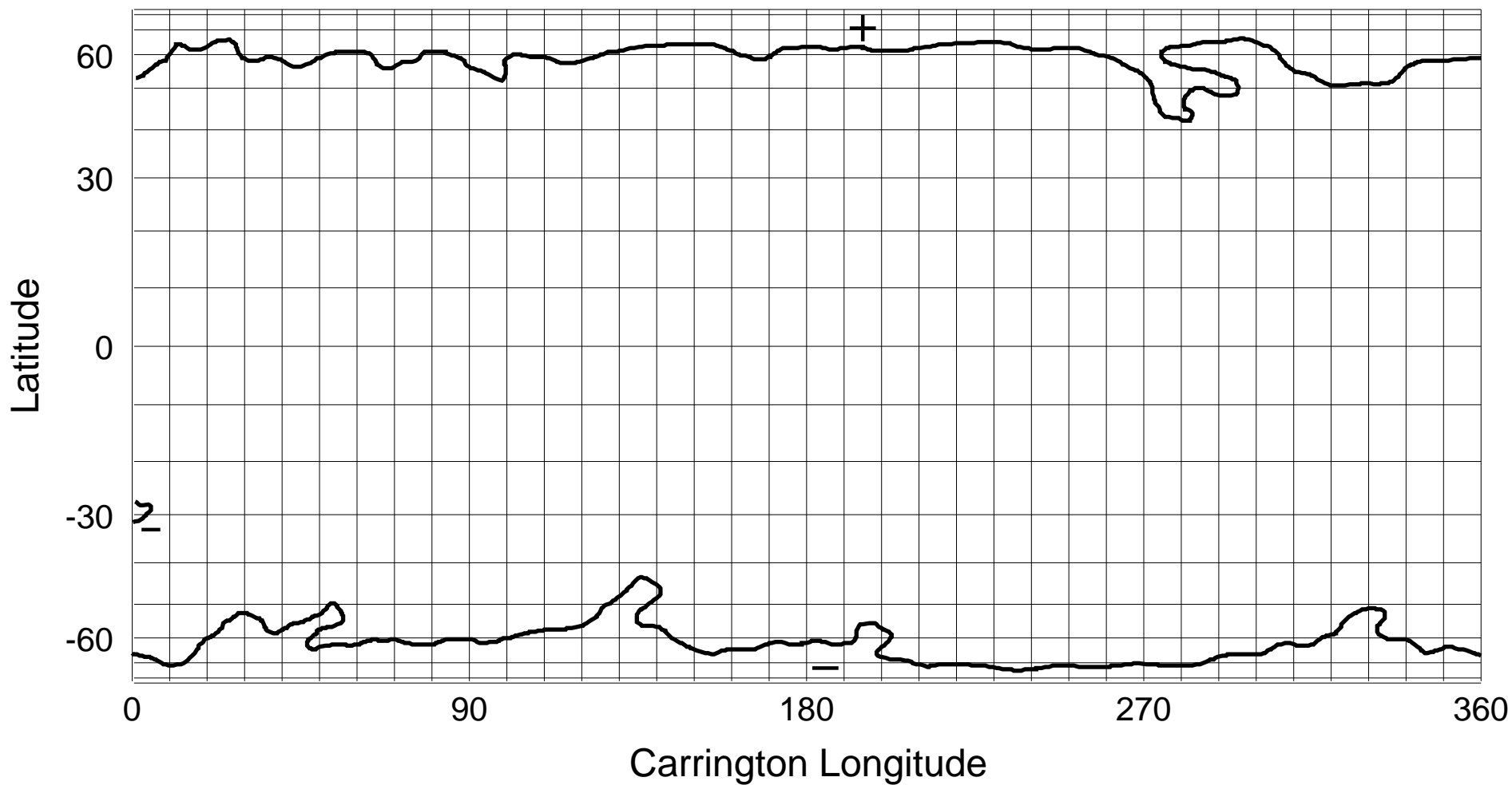
NSO/KP He I 1083 nm Coronal Hole Map: Carrington Rotation 1917
