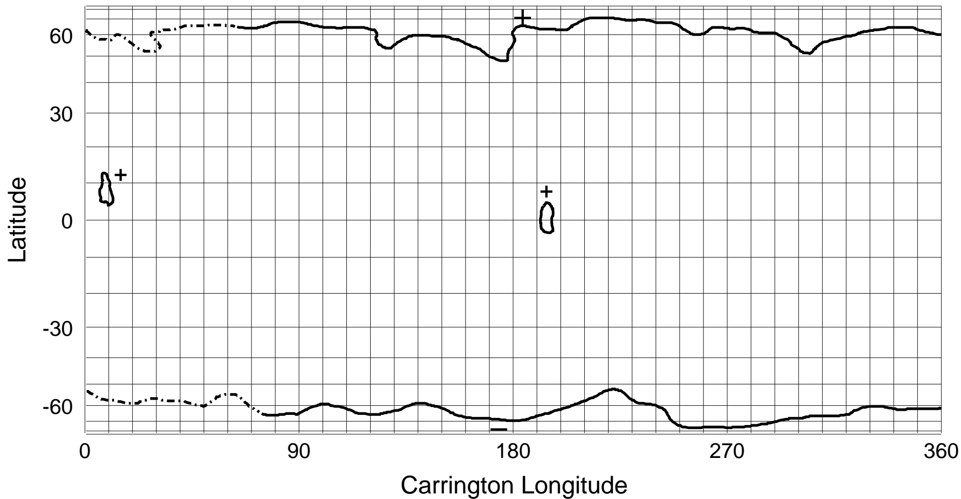
NSO/KP He I 1083 nm Coronal Hole Map: Carrington Rotation 1919
