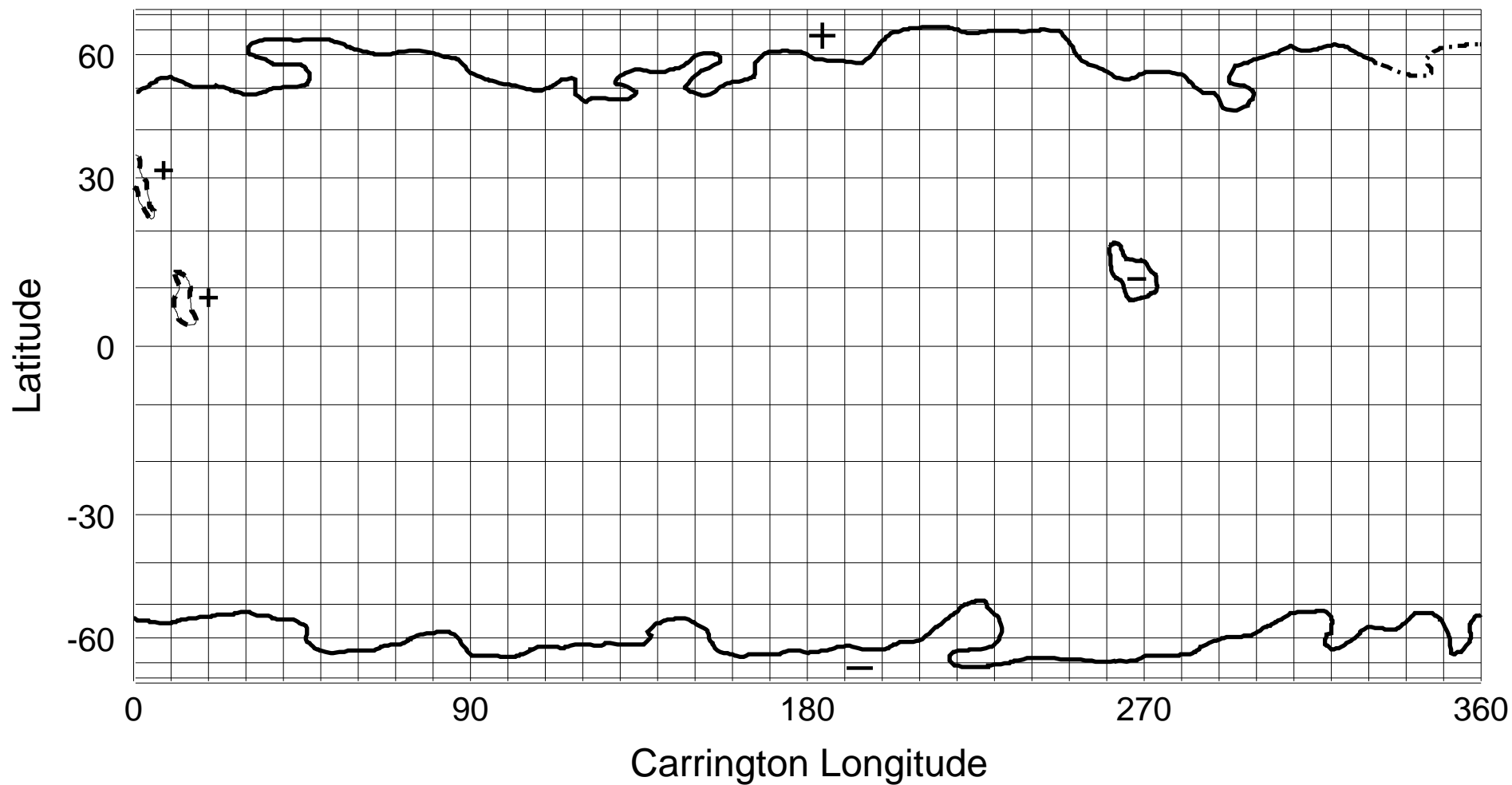
NSO/KP He I 1083 nm Coronal Hole Map: Carrington Rotation 1920
