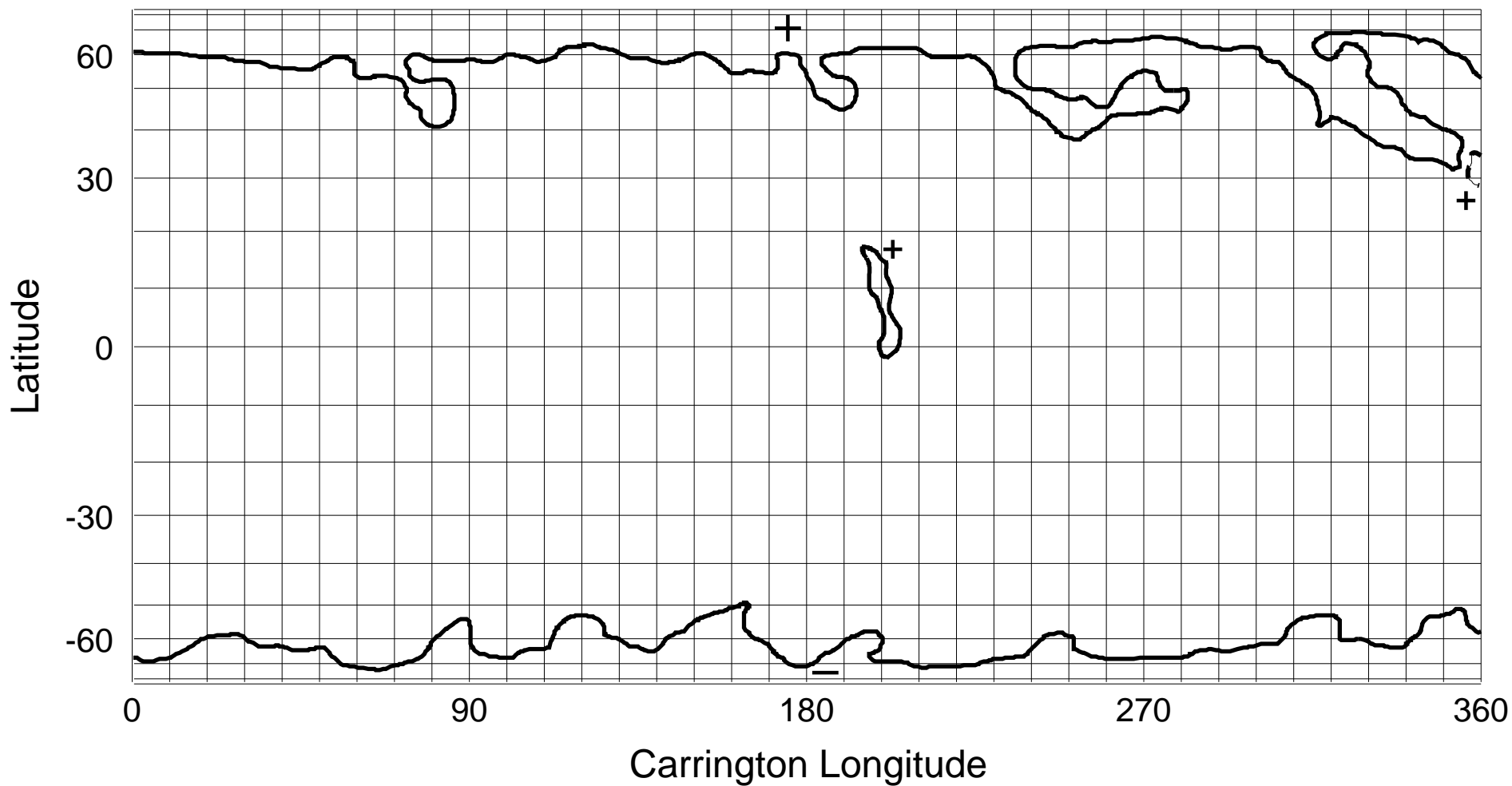
NSO/KP He I 1083 nm Coronal Hole Map: Carrington Rotation 1921
