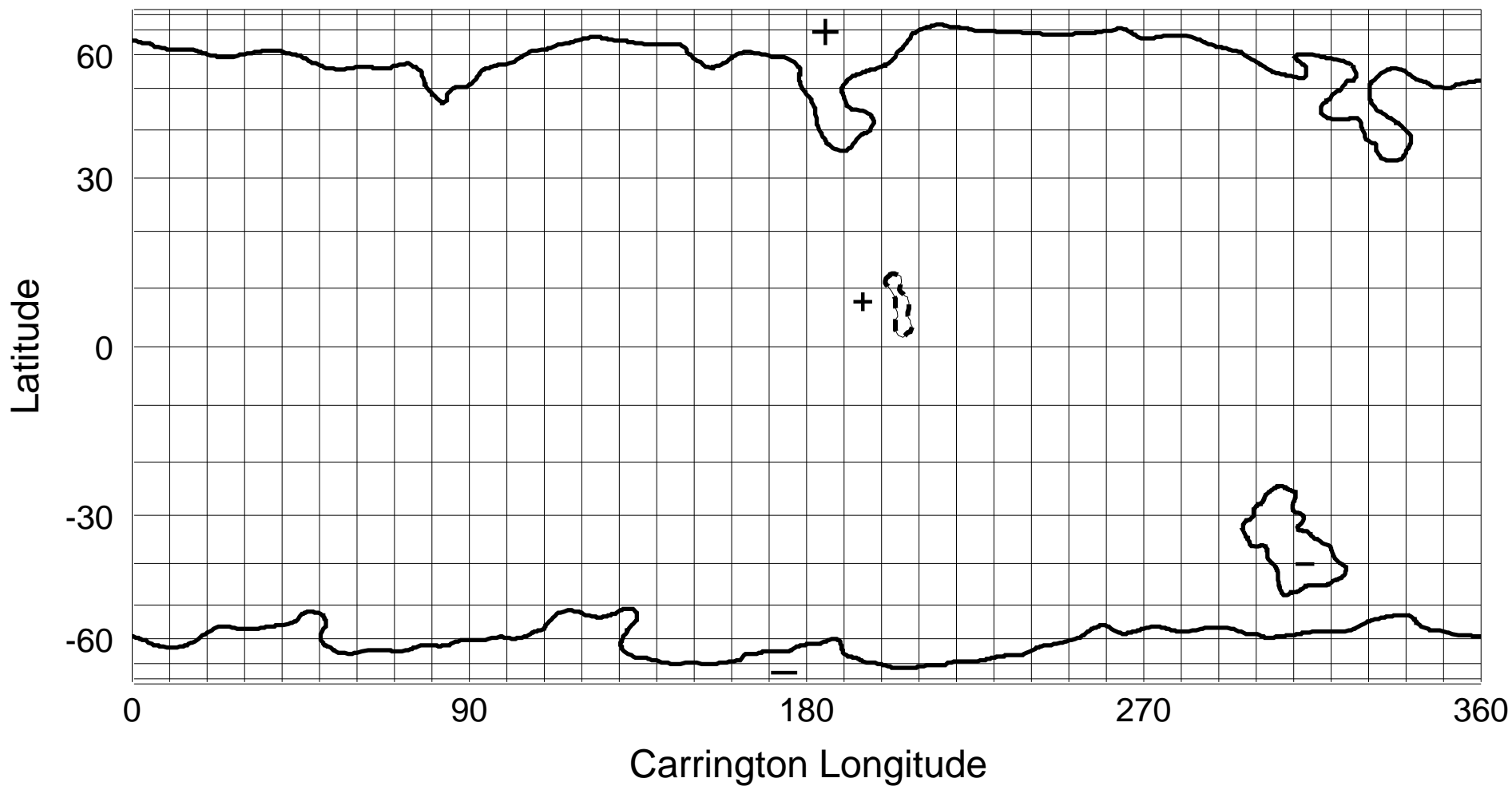
NSO/KP He I 1083 nm Coronal Hole Map: Carrington Rotation 1922
