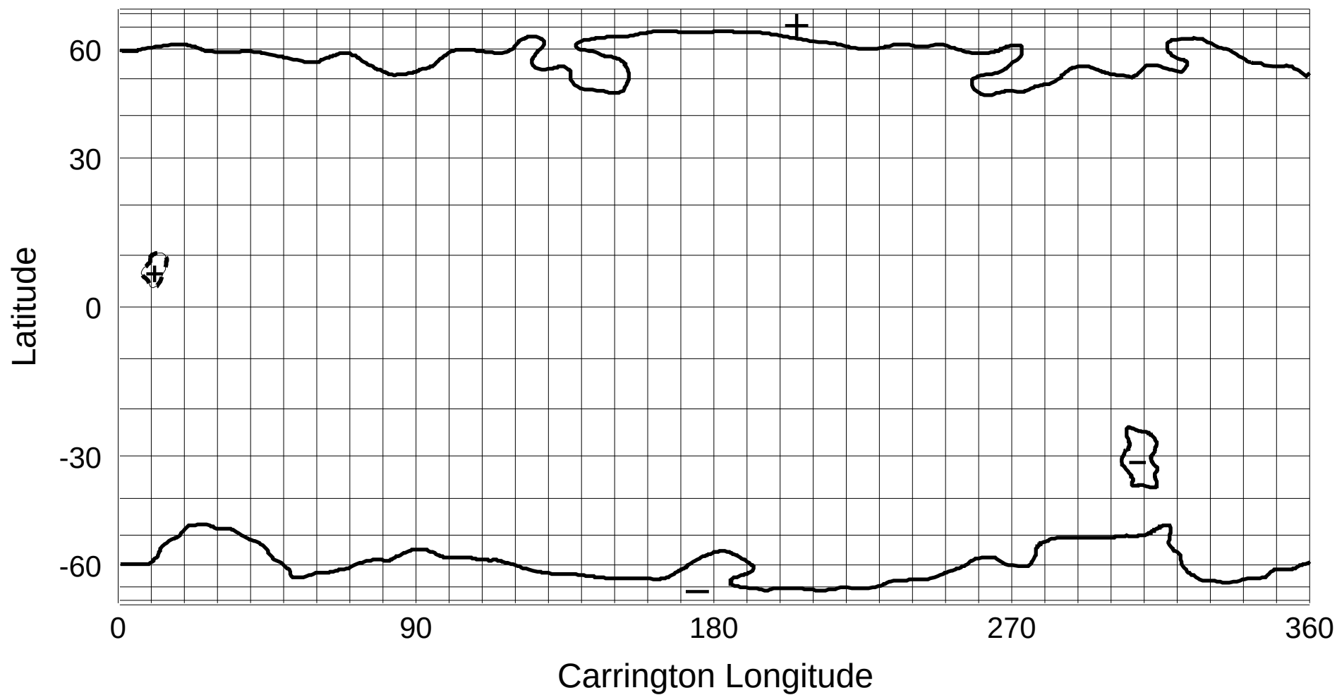
NSO/KP He I 1083 nm Coronal Hole Map: Carrington Rotation 1923
