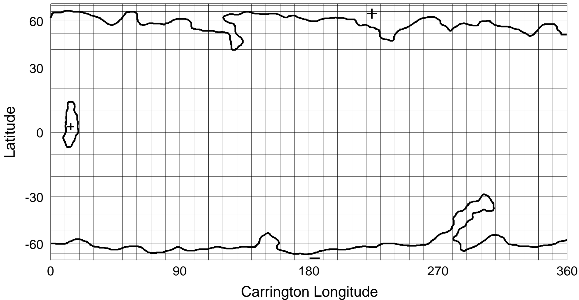
NSO/KP He I 1083 nm Coronal Hole Map: Carrington Rotation 1924
