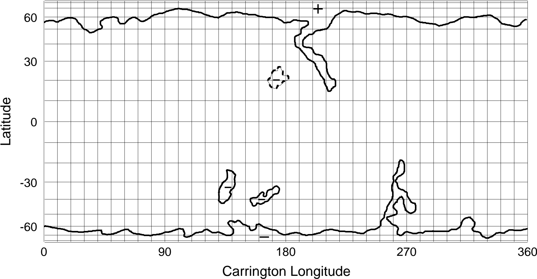
NSO/KP He I 1083 nm Coronal Hole Map: Carrington Rotation 1925
