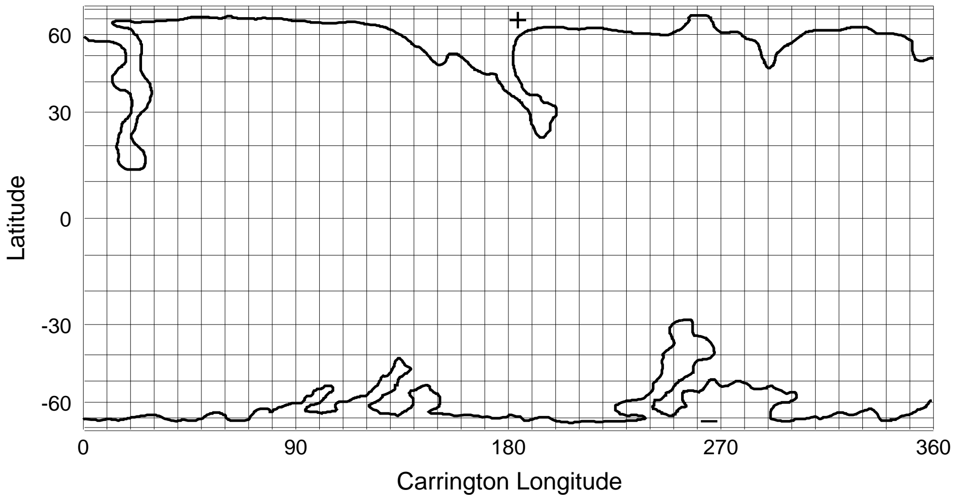
NSO/KP He I 1083 nm Coronal Hole Map: Carrington Rotation 1926
