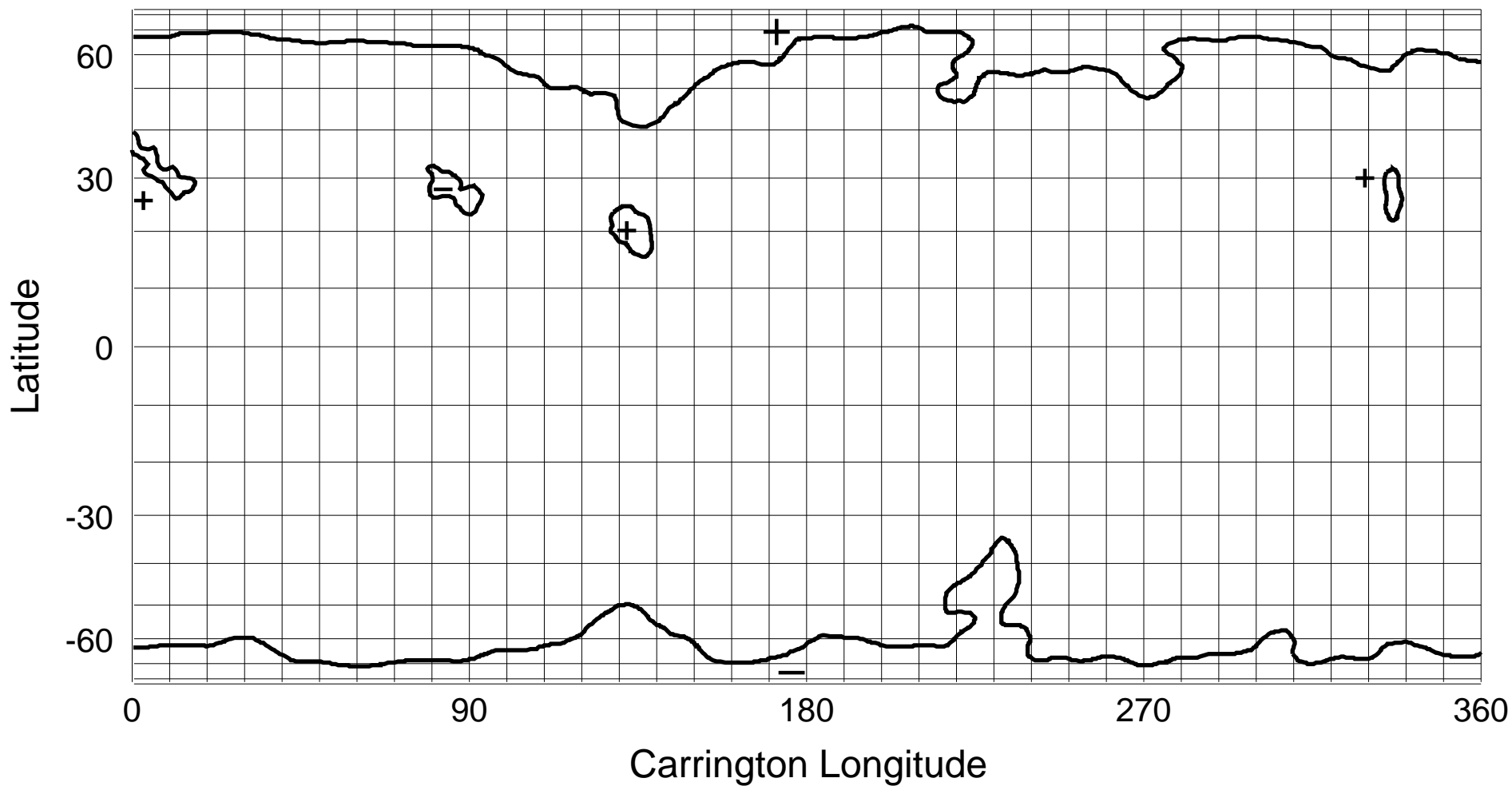
NSO/KP He I 1083 nm Coronal Hole Map: Carrington Rotation 1927
