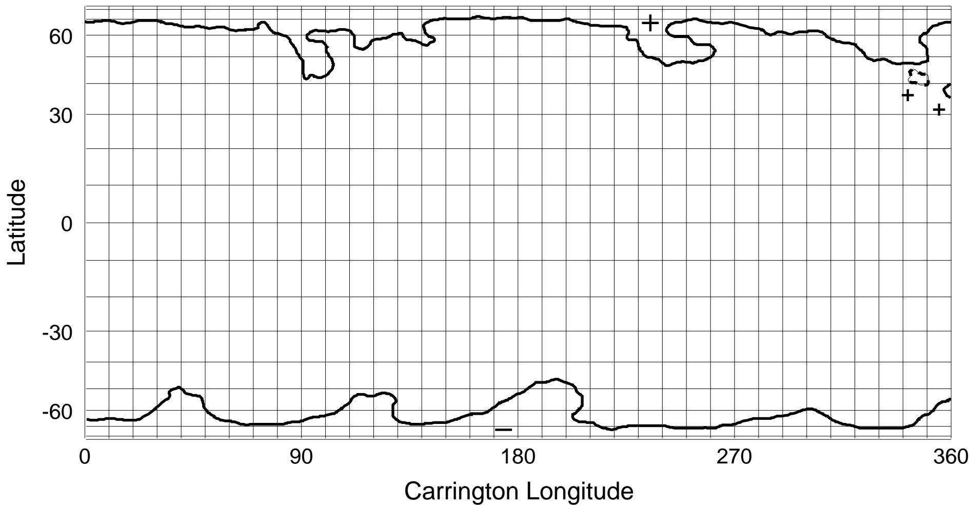
NSO/KP He I 1083 nm Coronal Hole Map: Carrington Rotation 1928
