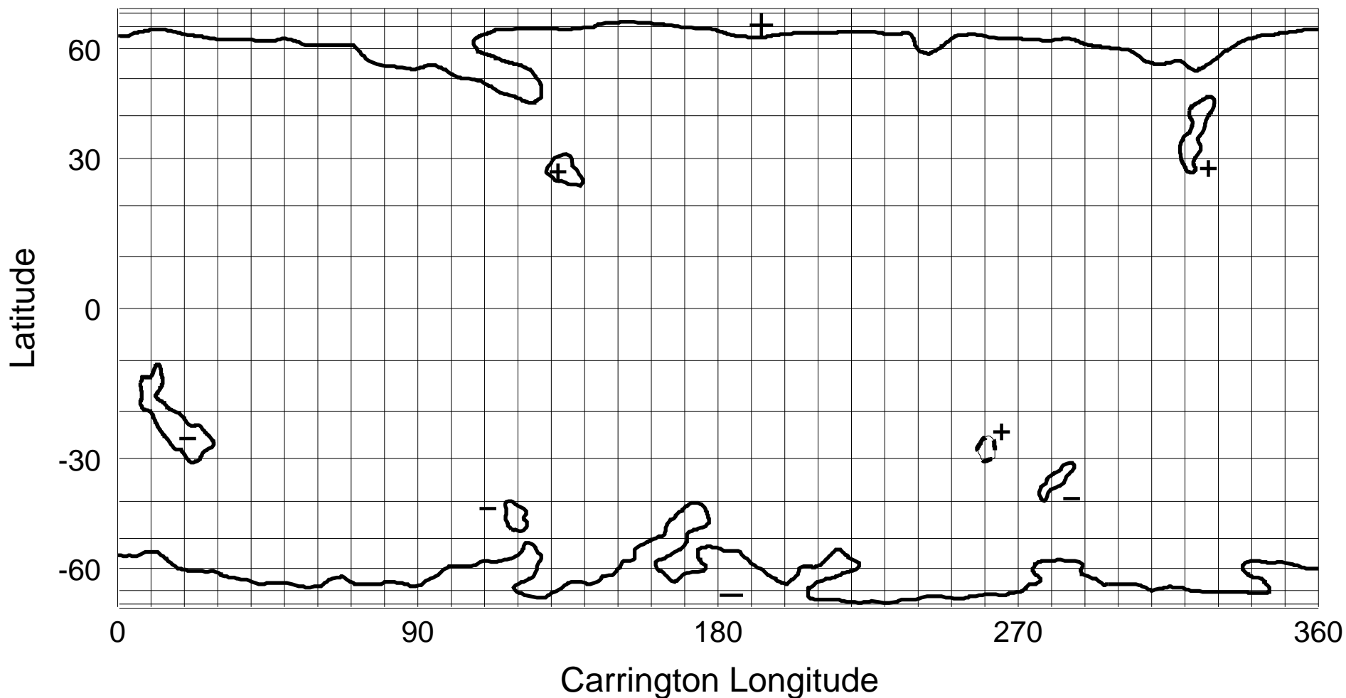
NSO/KP He I 1083 nm Coronal Hole Map: Carrington Rotation 1929
