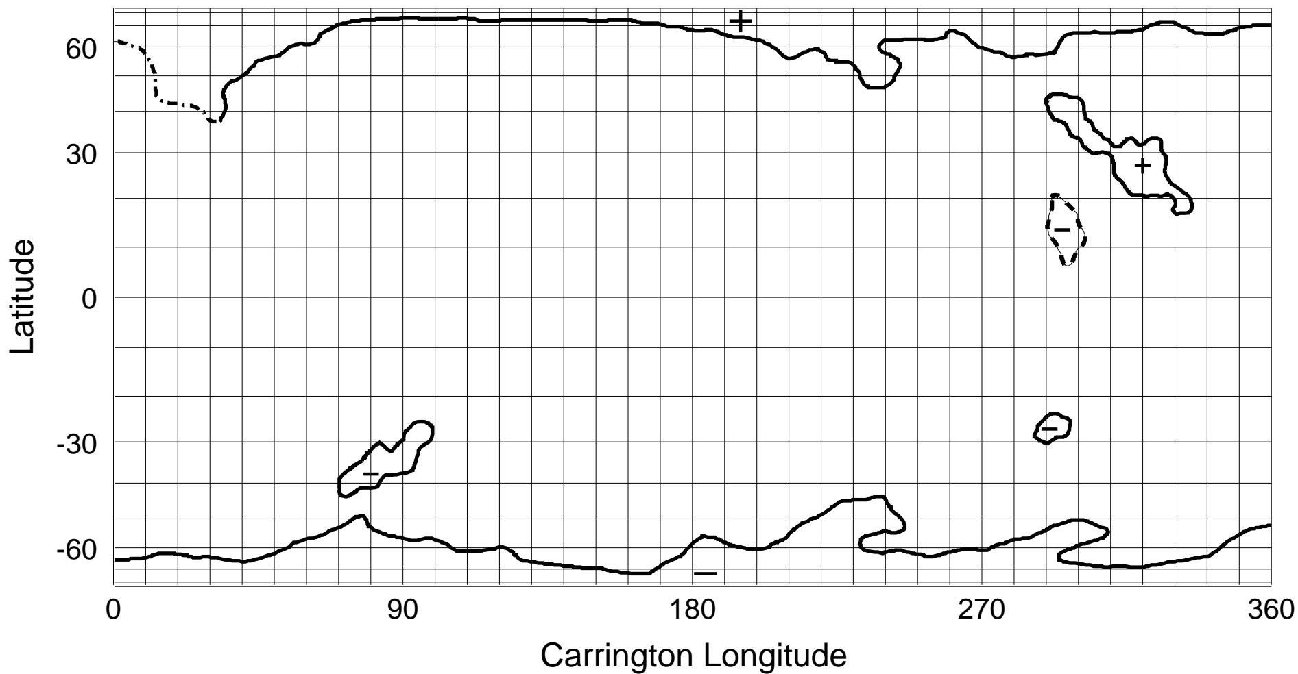
NSO/KP He I 1083 nm Coronal Hole Map: Carrington Rotation 1931
