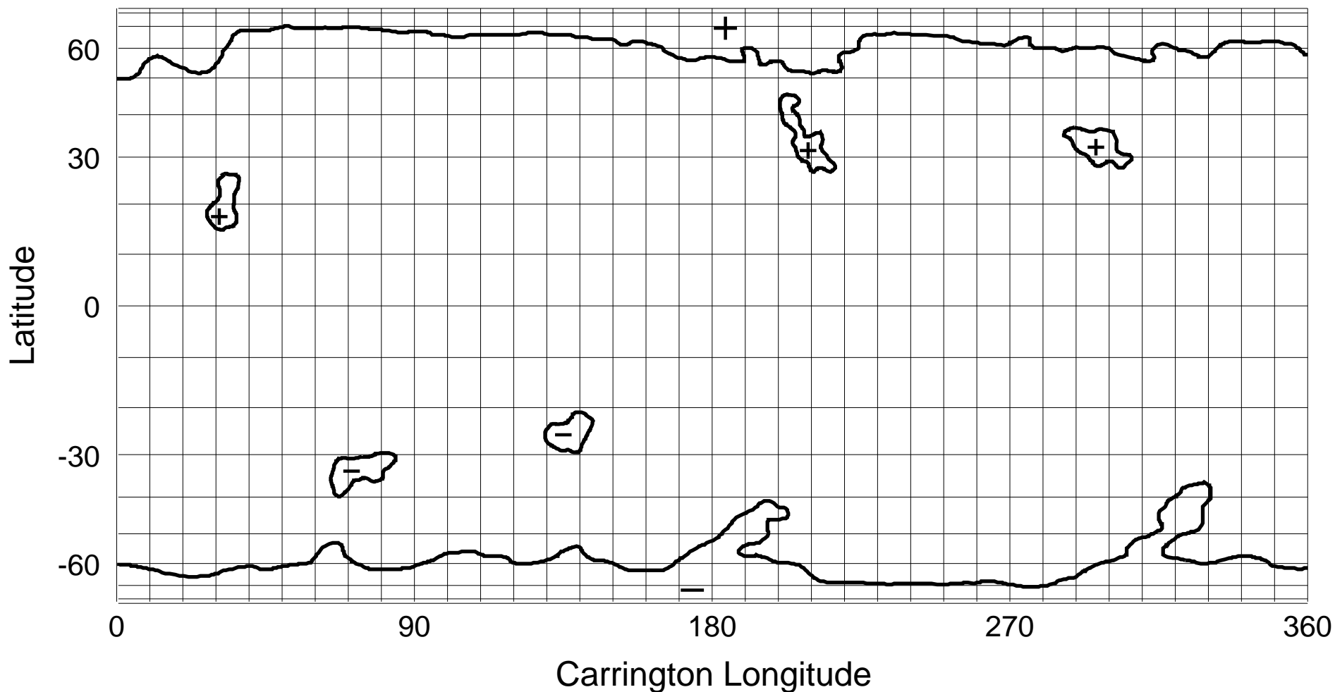
NSO/KP He I 1083 nm Coronal Hole Map: Carrington Rotation 1932
