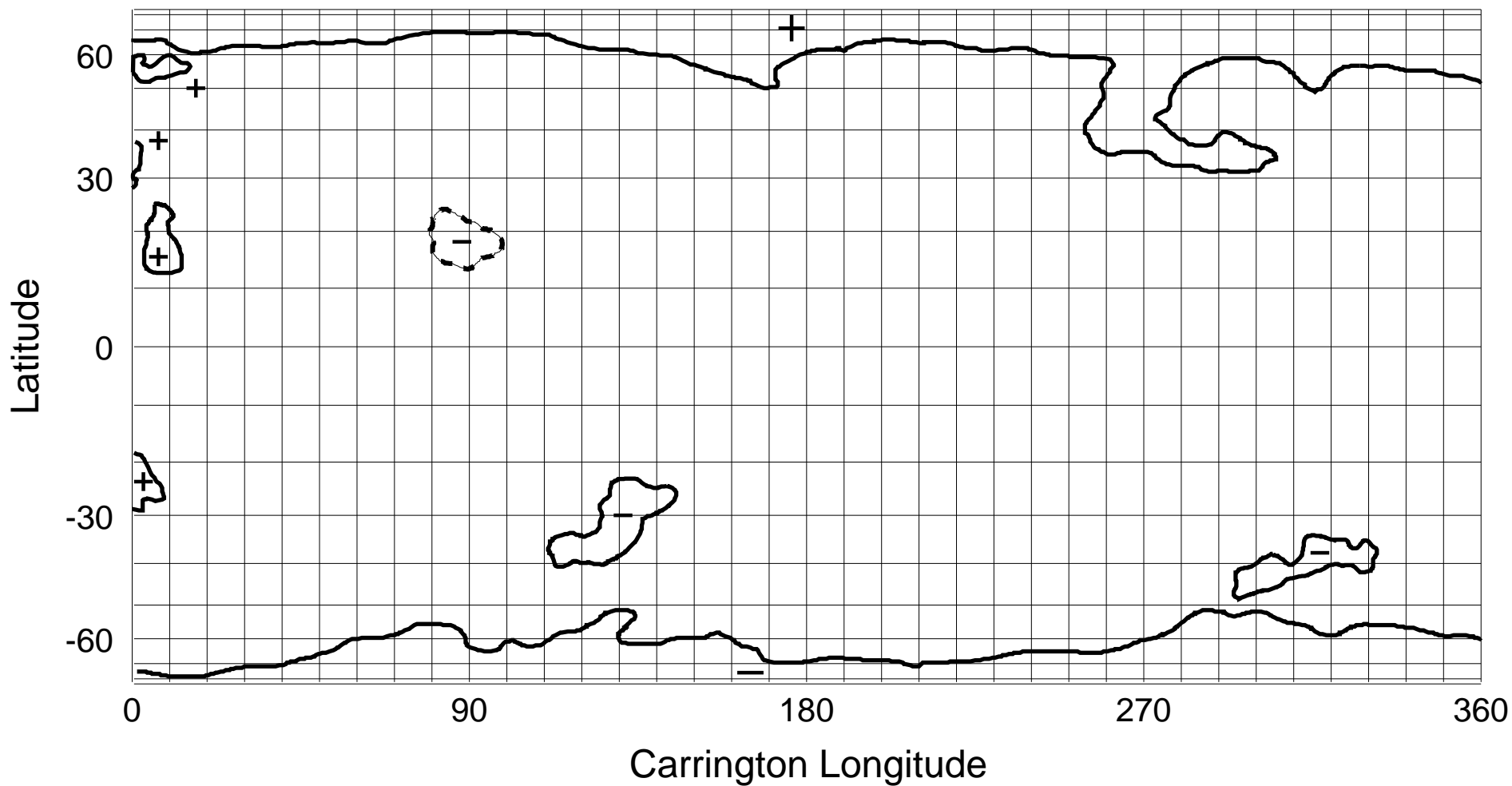
NSO/KP He I 1083 nm Coronal Hole Map: Carrington Rotation 1933
