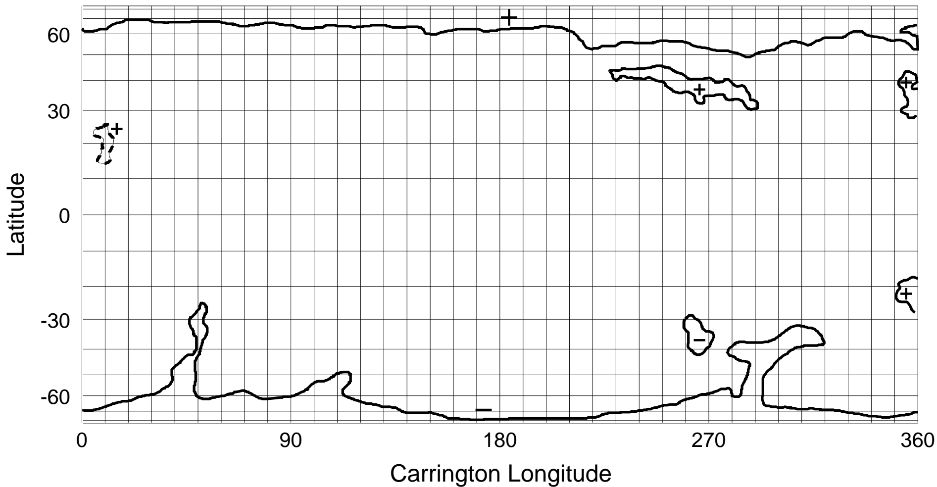
NSO/KP He I 1083 nm Coronal Hole Map: Carrington Rotation 1934
