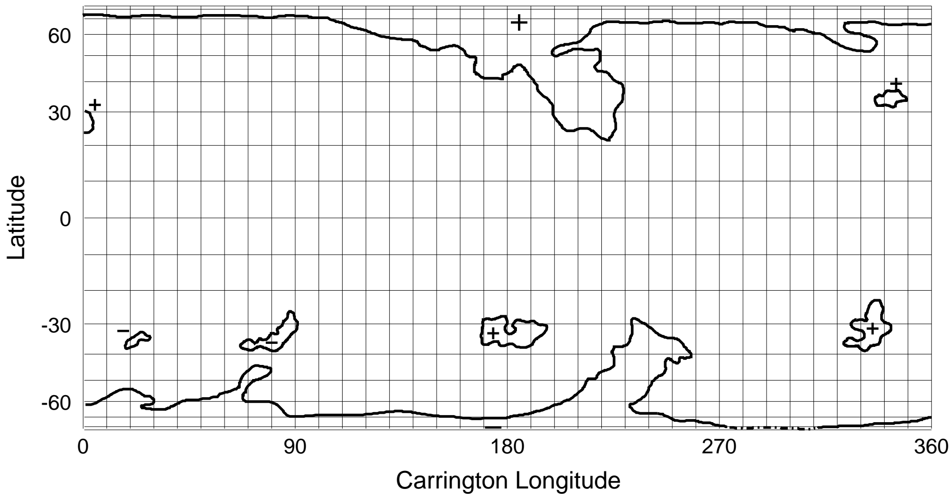
NSO/KP He I 1083 nm Coronal Hole Map: Carrington Rotation 1936
