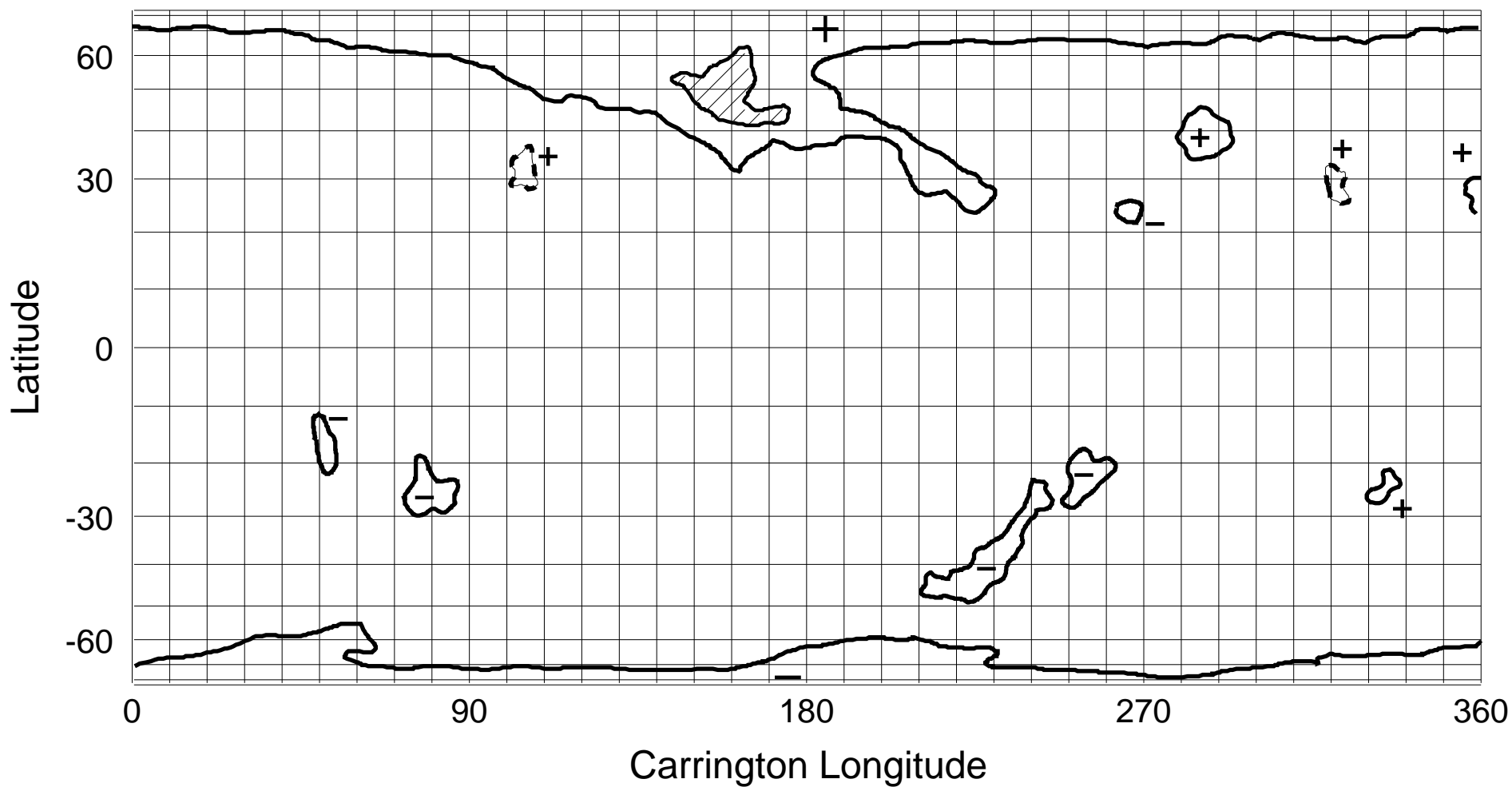
NSO/KP He I 1083 nm Coronal Hole Map: Carrington Rotation 1937
