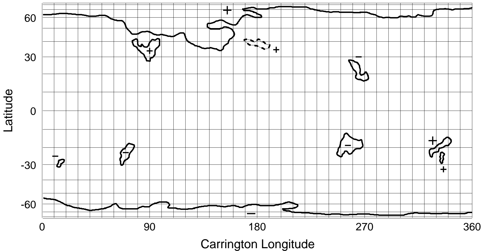
NSO/KP He I 1083 nm Coronal Hole Map: Carrington Rotation 1938
