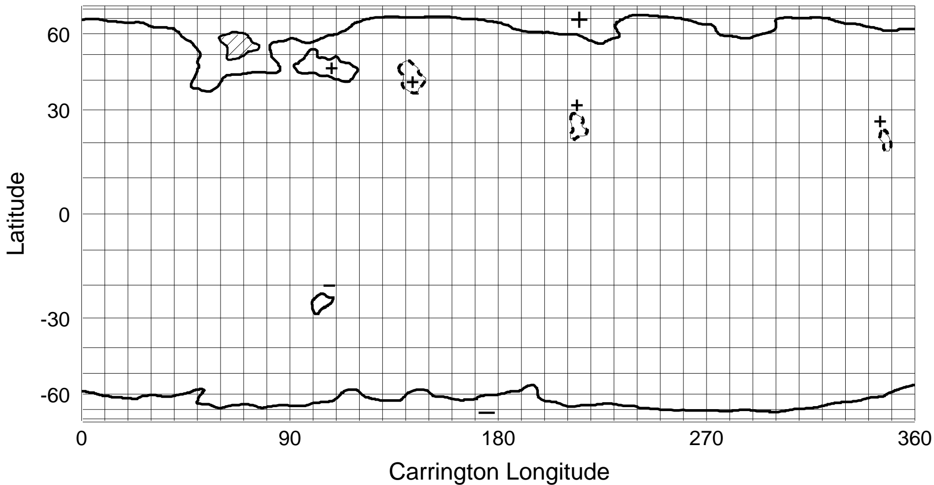
NSO/KP He I 1083 nm Coronal Hole Map: Carrington Rotation 1939
