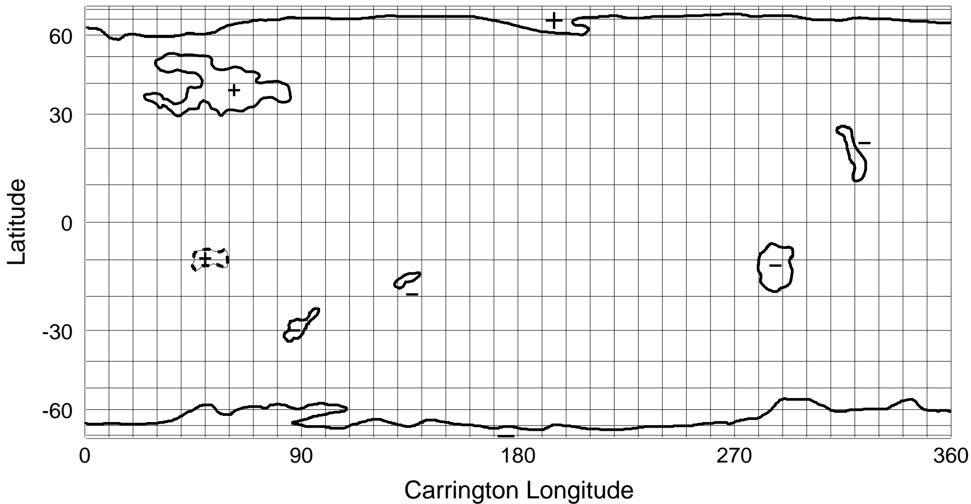
NSO/KP He I 1083 nm Coronal Hole Map: Carrington Rotation 1941
