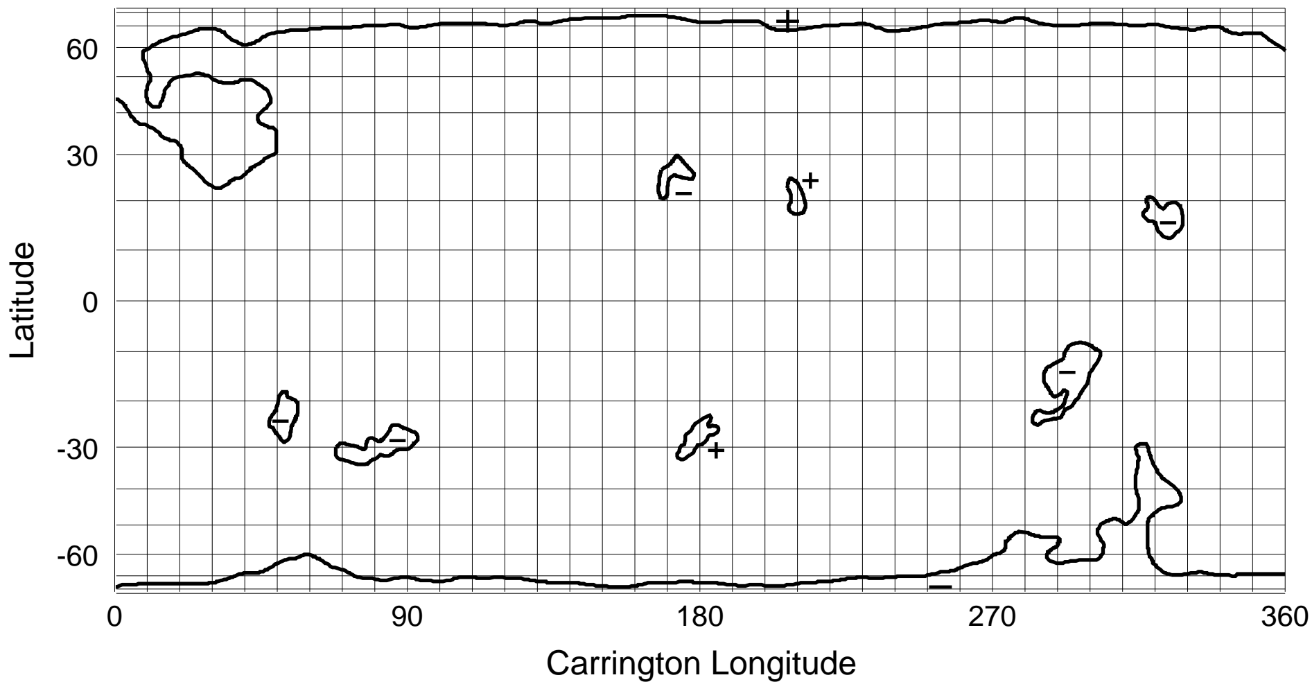
NSO/KP He I 1083 nm Coronal Hole Map: Carrington Rotation 1942
