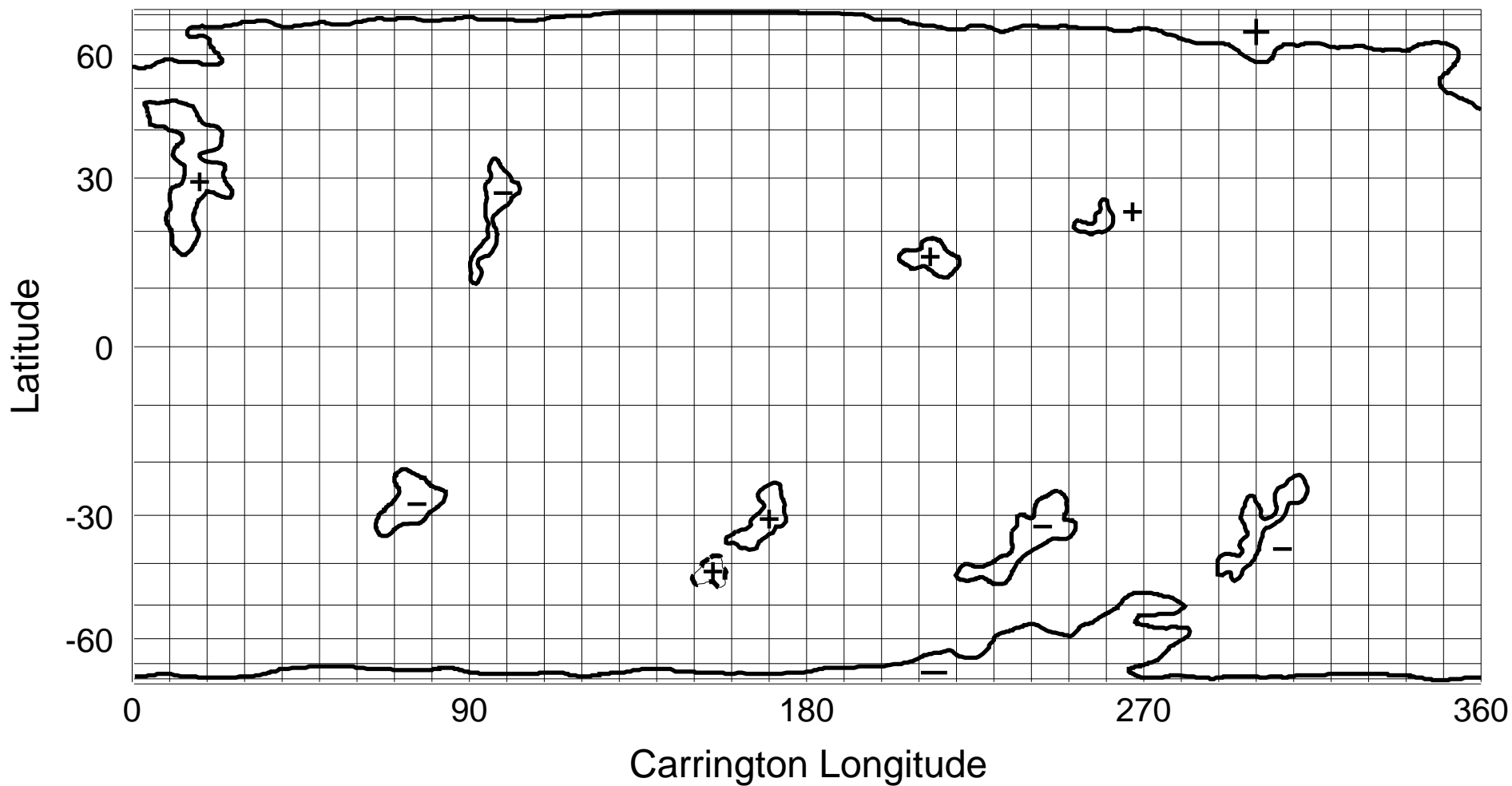
NSO/KP He I 1083 nm Coronal Hole Map: Carrington Rotation 1943
